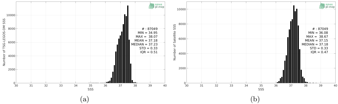
Figure 2: Histograms of SSS from TSG-LEGOS-DM (a) and SMOS-L4-CATDS-CECOS-IFREMER-V2-WEEKLY-0.5DEG (b) considering all match-up pairs per bins of 0.1 over the SPURS 1 Pi-MEP region and for the full satellite product period.
