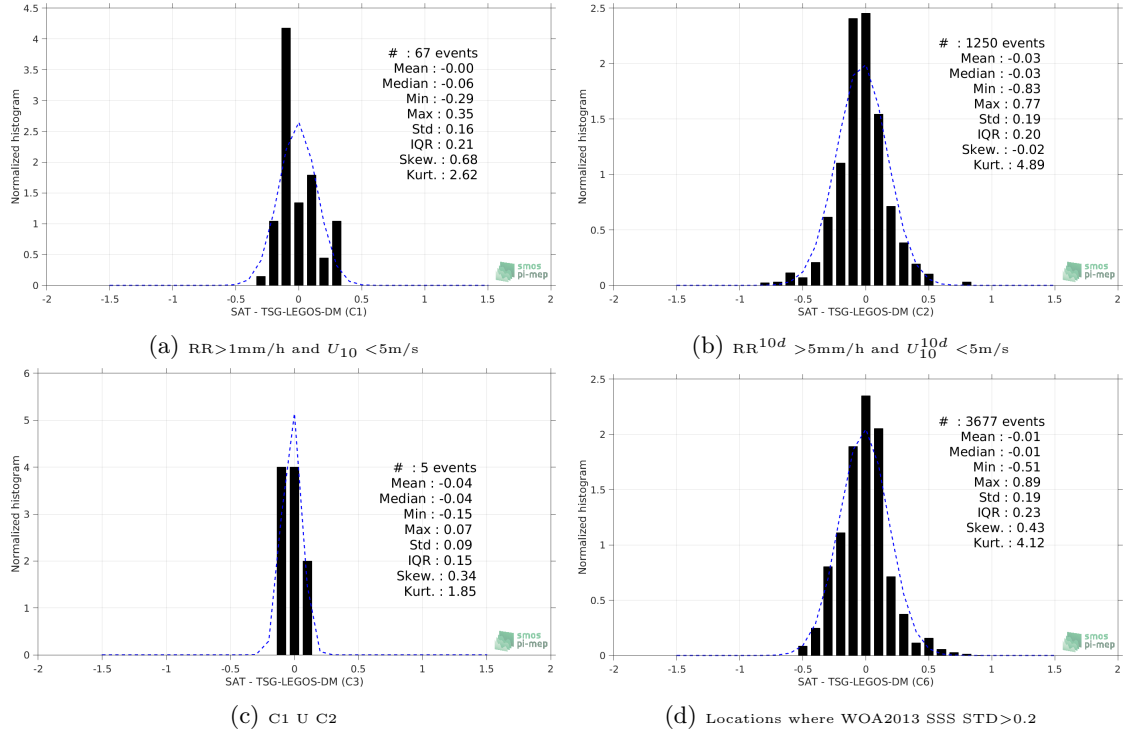
Figure 13: Normalized histogram of \Delta SSS (SMOS-L4-CATDS-CECOS-IFREMER-V2-WEEKLY-0.5DEG - TSG-LEGOS-DM) for 6 different subdatasets corresponding to: RR > 1mm/h and U_{10} < 5 m/s (a), RR^{10d} > 5 mm/h and U_{10}^{10d} < 5 m/s (b), C1 U C2 (c), Locations where WOA2013 SSS STD > 0.2 (d).
