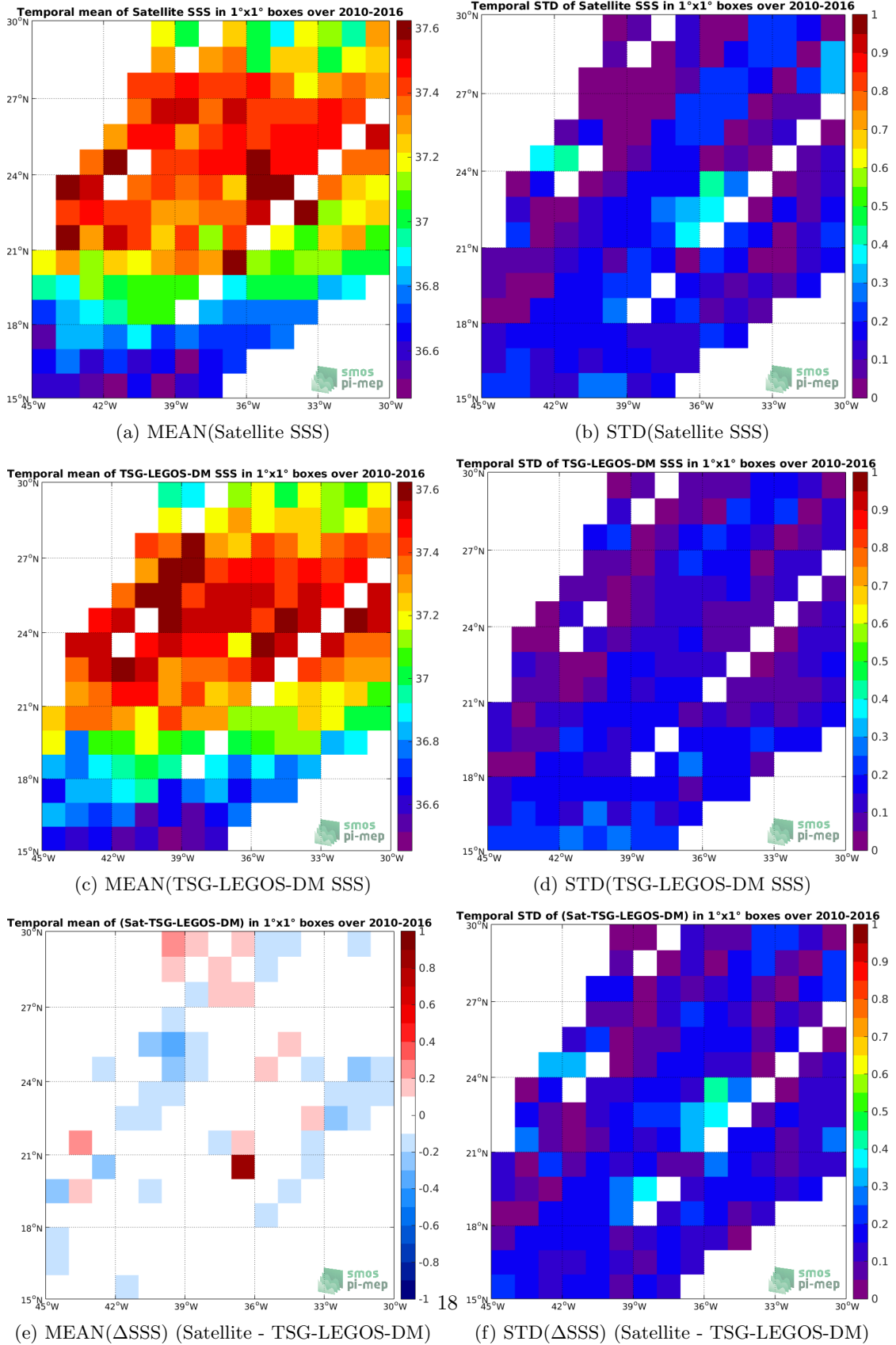
Figure 6: Temporal mean (left) and STD (right) of SSS from SMOS-L4-CATDS-CECOS-IFREMER-V2-WEEKLY-0.5DEG (top), TSG-LEGOS-DM (middle), and of \Delta SSS (Satellite - TSG-LEGOS-DM). Only match-up pairs are used to generate these maps.
