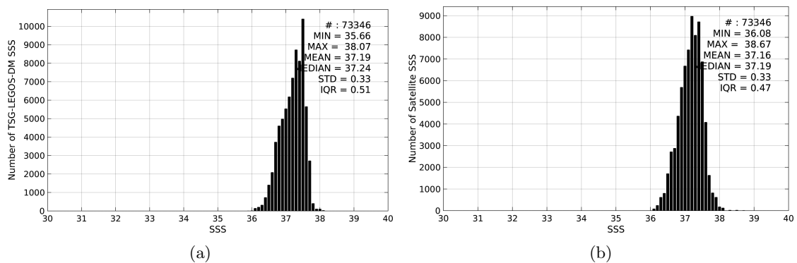
Figure 2: Histograms of SSS from TSG-LEGOS-DM (a) and SMOS-L4-CATDS-CECOS-IFREMER-V2-WEEKLY-0.5DEG (b) considering all match-up pairs per bins of 0.1 over the SPURS 1 Pi-MEP region and for the full satellite product period.
