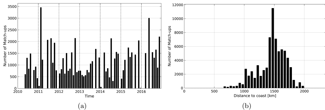
Figure 1: Number of match-ups between TSG-LEGOS-DM and SMOS-L4-CATDS-CECOS-IFREMER-V2-WEEKLY-0.5DEG SSS as a function of time (a) and as function of the distance to coast (b) over the SPURS 1 Pi-MEP region and for the full satellite product period.
