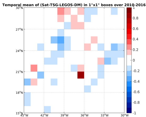
Figure 6: Temporal mean (left) and STD (right) of SSS from SMOS-L4-CATDS-CECOS-IFREMER-V2-WEEKLY-0.5DEG (top), TSG-LEGOS-DM (middle), and of \Delta SSS (Satellite - TSG-LEGOS-DM). Only match-up pairs are used to generate these maps.
