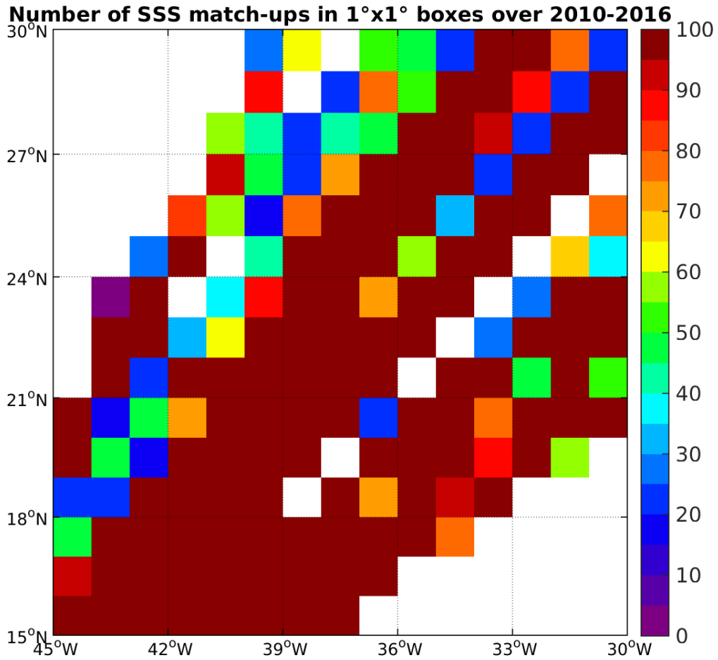
Figure 4: Number of SSS match-ups between TSG-LEGOS-DM SSS and the SMOS-L4-CATDS-CECOS-IFREMER-V2-WEEKLY-0.5DEG SSS product for the SPURS 1 Pi-MEP region over 1°x1° boxes and for the full satellite product period.
