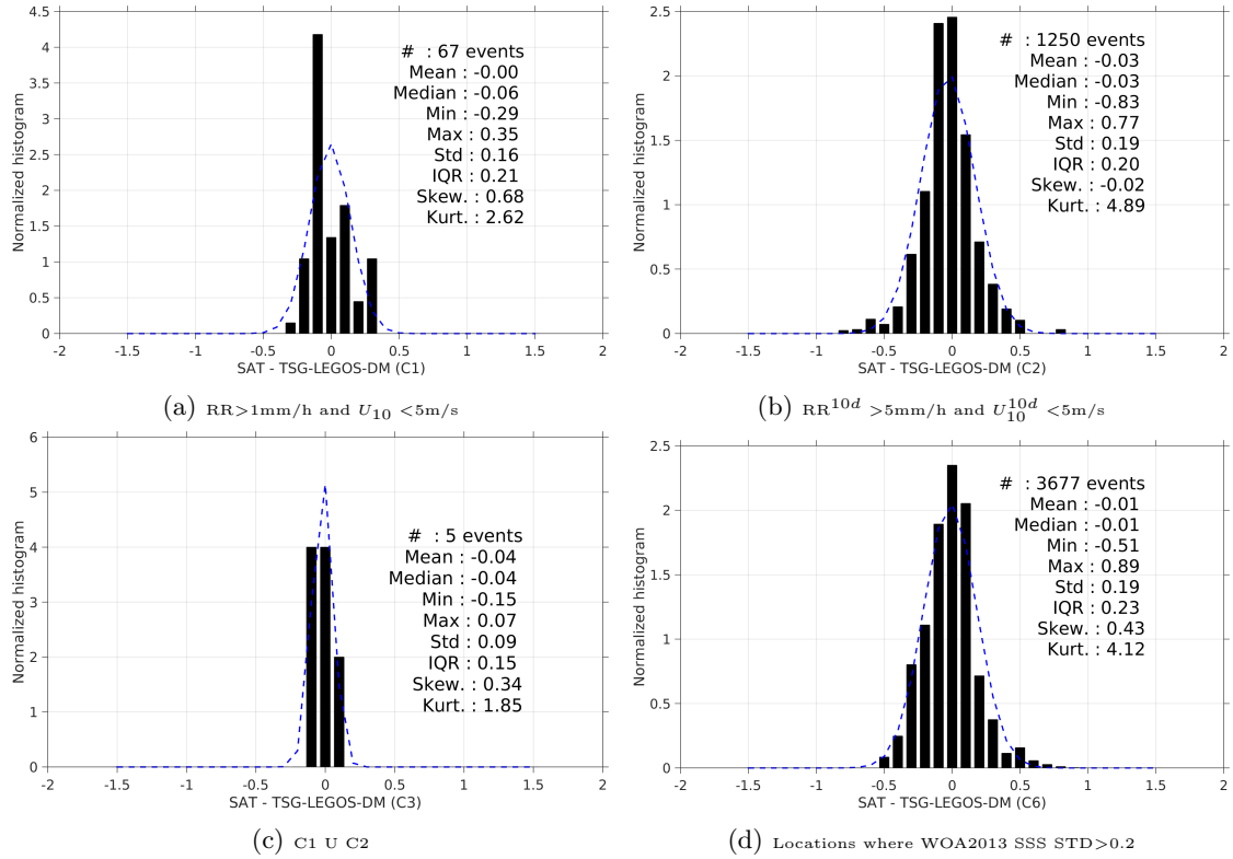
Figure 13: Normalized histogram of \Delta\text{SSS} (SMOS-L4-CATDS-CECOS-IFREMER-V2-WEEKLY-0.5DEG - TSG-LEGOS-DM) for 6 different subdatasets corresponding to: RR > 1\text{mm/h} and U_{10} < 5\text{m/s} (a), RR^{10d} > 5\text{mm/h} and U_{10}^{10d} < 5\text{m/s} (b), C1 U C2 (c), Locations where WOA2013 SSS STD > 0.2 (d).
