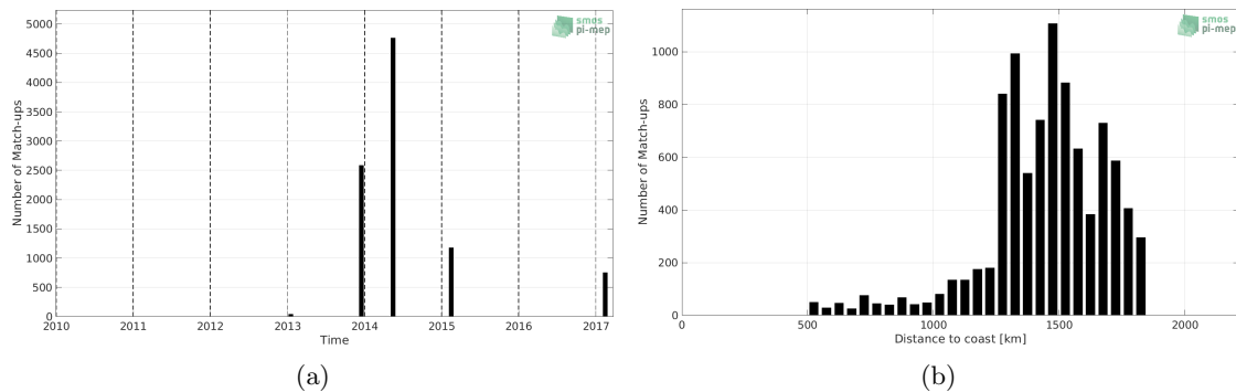
Figure 1: Number of match-ups between TSG (GOSUD-Sailing-ship) and SMOS L4 v2 Weekly (CATDS-CECOS-IFREMER) SSS as a function of time (a) and as function of the distance to coast (b) over the SPURS 1 Pi-MEP region and for the full satellite product period.
