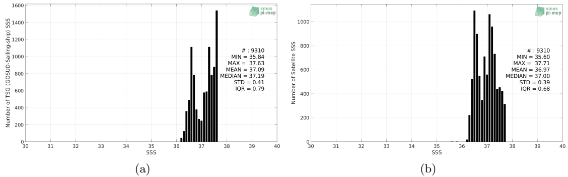
Figure 2: Histograms of SSS from TSG (GOSUD-Sailing-ship) (a) and SMOS L4 v2 Weekly (CATDS-CECOS-IFREMER) (b) considering all match-up pairs per bins of 0.1 over the SPURS 1 Pi-MEP region and for the full satellite product period.
