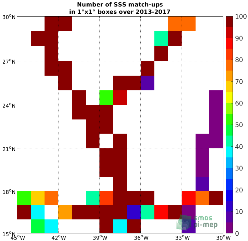
Figure 4: Number of SSS match-ups between TSG (GOSUD-Sailing-ship) SSS and the SMOS L4 v2 Weekly (CATDS-CECOS-IFREMER) SSS product for the SPURS 1 Pi-MEP region over 1^\circ \times 1^\circ boxes and for the full satellite product period.
