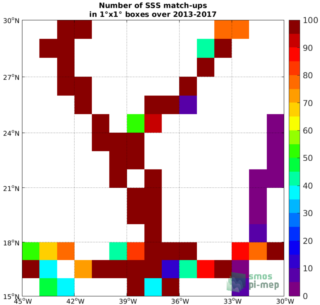
Figure 4: Number of SSS match-ups between TSG (GOSUD-Sailing-ship) SSS and the SMOS L4 v2 Weekly (CATDS-CECOS-IFREMER) SSS product for the SPURS 1 Pi-MEP region over 1°x1° boxes and for the full satellite product period.
