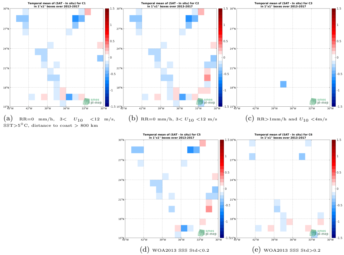
Figure 12: Temporal mean gridded over spatial boxes of size 1^{\circ} \times 1^{\circ} of \Delta\text{SSS} (SMOS L4 v2 Weekly (CATDS-CECOS-IFREMER) - TSG (GOSUD-Sailing-ship)) for 5 different subdatasets corresponding to: RR=0 mm/h, 3 < U_{10} < 12 m/s, SST > 5^{\circ}\text{C} , distance to coast > 800 km (a), RR=0 mm/h, 3 < U_{10} < 12 m/s (b), RR > 1\text{mm/h} and U_{10} < 4\text{m/s} (c), \text{WOA}_{2013} \text{ SSS Std} < 0.2 (d), \text{WOA}_{2013} \text{ SSS Std} > 0.2 (e).
