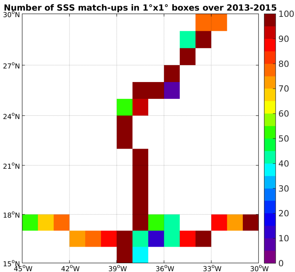
Figure 4: Number of SSS match-ups between TSG-GOSUD-Sailing-ship SSS and the SMOS-L4-CATDS-CECOS-IFREMER-V2-WEEKLY-0.5DEG SSS product for the SPURS 1 Pi-MEP region over 1°x1° boxes and for the full satellite product period.
