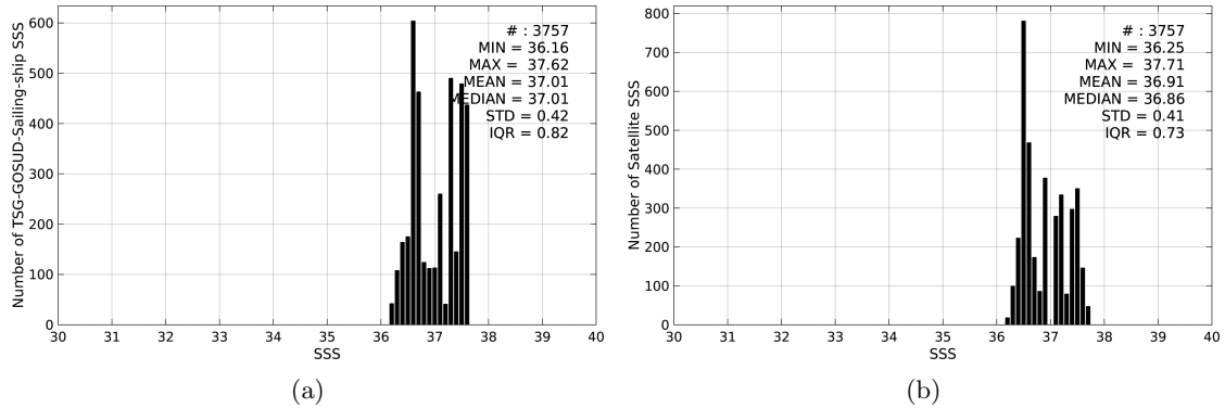
Figure 2: Histograms of SSS from TSG-GOSUD-Sailing-ship (a) and SMOS-L4-CATDS-CECOS-IFREMER-V2-WEEKLY-0.5DEG (b) considering all match-up pairs per bins of 0.1 over the SPURS 1 Pi-MEP region and for the full satellite product period.
