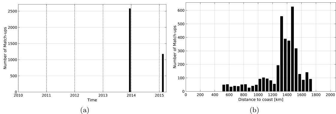
Figure 1: Number of match-ups between TSG-GOSUD-Sailing-ship and SMOS-L4-CATDS-CECOS-IFREMER-V2-WEEKLY-0.5DEG SSS as a function of time (a) and as function of the distance to coast (b) over the SPURS 1 Pi-MEP region and for the full satellite product period.
