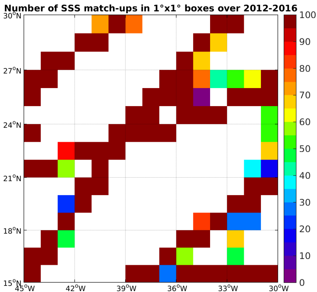
Figure 4: Number of SSS match-ups between TSG-GOSUD-Research-vessel SSS and the SMOS-L4-CATDS-CECOS-IFREMER-V2-WEEKLY-0.5DEG SSS product for the SPURS 1 Pi-MEP region over 1°x1° boxes and for the full satellite product period.
