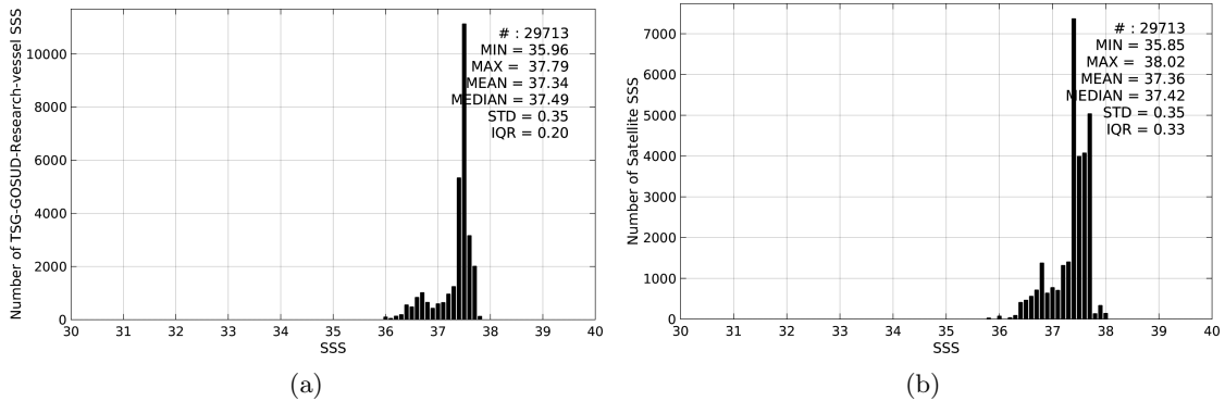
Figure 2: Histograms of SSS from TSG-GOSUD-Research-vessel (a) and SMOS-L4-CATDS-CECOS-IFREMER-V2-WEEKLY-0.5DEG (b) considering all match-up pairs per bins of 0.1 over the SPURS 1 Pi-MEP region and for the full satellite product period.
