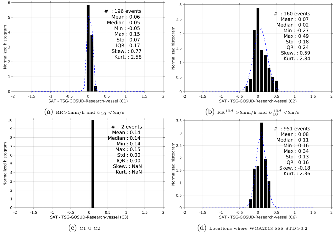
Figure 13: Normalized histogram of \Delta\text{SSS} (SMOS-L4-CATDS-CECOS-IFREMER-V2-WEEKLY-0.5DEG - TSG-GOSUD-Research-vessel) for 6 different subdatasets corresponding to: RR > 1mm/h and U_{10} < 5\text{m/s} (a), RR^{10d} > 5\text{mm/h} and U_{10}^{10d} < 5\text{m/s} (b), C1 U C2 (c), Locations where WOA2013 SSS STD > 0.2 (d).
