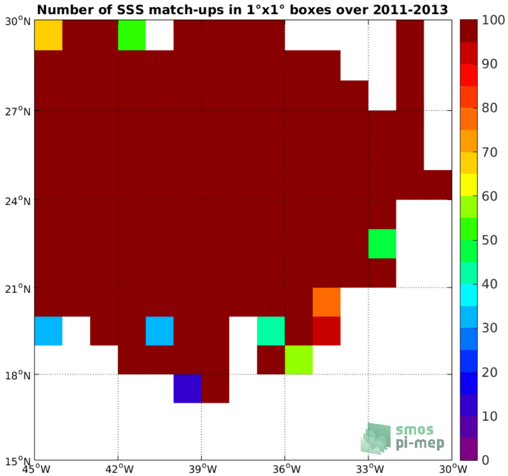
Figure 3: Number of SSS match-ups between Surface drifters SSS and the SMOS-L4-CATDS-CECOS-IFREMER-V2-WEEKLY-0.5DEG SSS product for the SPURS 1 Pi-MEP region over 1°x1° boxes and for the full satellite product period.
