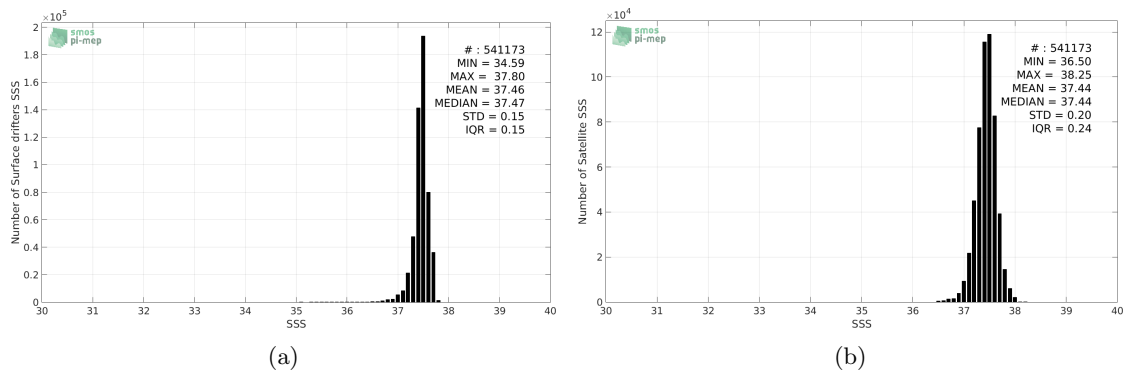
Figure 2: Histograms of SSS from Surface drifters (a) and SMOS-L4-CATDS-CECOS-IFREMER-V2-WEEKLY-0.5DEG (b) considering all match-up pairs per bins of 0.1 over the SPURS 1 Pi-MEP region and for the full satellite product period.
