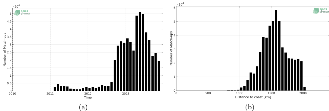
Figure 1: Number of match-ups between Surface drifters and SMOS-L4-CATDS-CECOS-IFREMER-V2-WEEKLY-0.5DEG SSS as a function of time (a) and as function of the distance to coast (b) over the SPURS 1 Pi-MEP region and for the full satellite product period.
