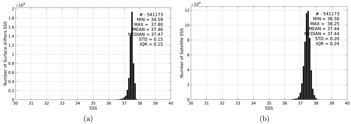
Figure 2: Histograms of SSS from Surface drifters (a) and SMOS-L4-CATDS-CECOS-IFREMER-V2-WEEKLY-0.5DEG (b) considering all match-up pairs per bins of 0.1 over the SPURS 1 Pi-MEP region and for the full satellite product period.
