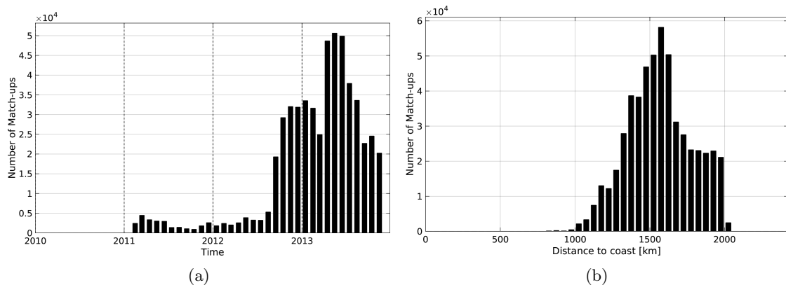
Figure 1: Number of match-ups between Surface drifters and SMOS-L4-CATDS-CECOS-IFREMER-V2-WEEKLY-0.5DEG SSS as a function of time (a) and as function of the distance to coast (b) over the SPURS 1 Pi-MEP region and for the full satellite product period.
