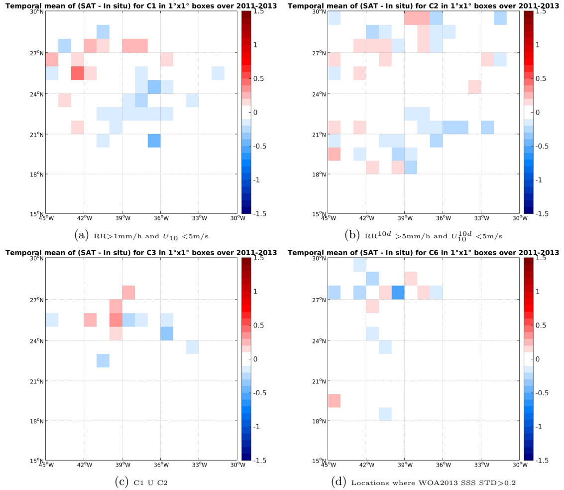
Figure 11: Temporal mean gridded over spatial boxes of size 1^\circ \times 1^\circ of \Delta SSS (SMOS-L4-CATDS-CECOS-IFREMER-V2-WEEKLY-0.5DEG - Surface drifters) for 4 different subdatasets corresponding to: RR > 1\text{mm/h} and U_{10} < 5\text{m/s} (a), RR^{10d} > 5\text{mm/h} and U_{10}^{10d} < 5\text{m/s} (b), C1 U C2 (c), Locations where WOA2013 SSS STD > 0.2 (d).
