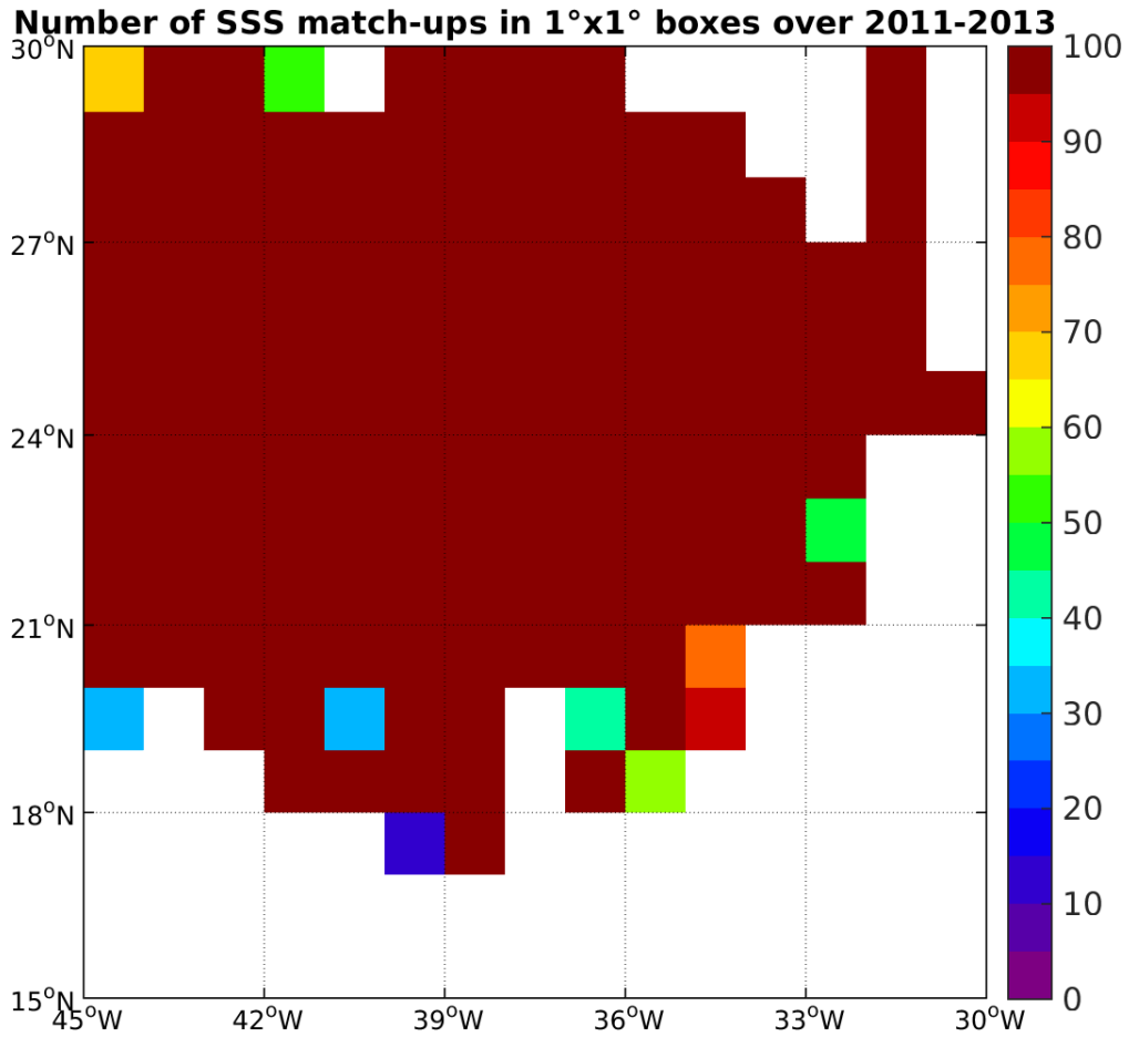
Figure 3: Number of SSS match-ups between Surface drifters SSS and the SMOS-L4-CATDS-CECOS-IFREMER-V2-WEEKLY-0.5DEG SSS product for the SPURS 1 Pi-MEP region over 1°x1° boxes and for the full satellite product period.
