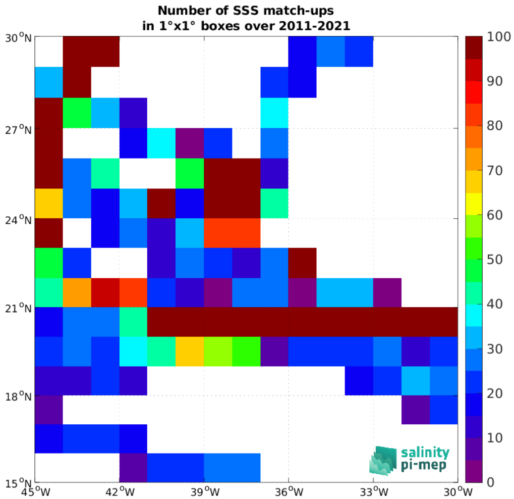
Figure 5: Number of SSS match-ups between TSG (SAMOS) SSS and the SMOS SSS L4 v2 - Daily (BEC) SSS product for the SPURS 1 Pi-MEP region over 1°x1° boxes and for the full satellite product period.
