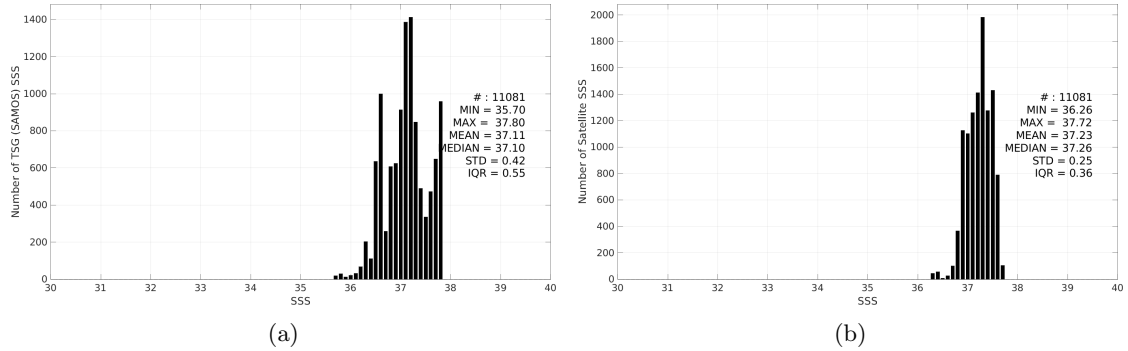
Figure 3: Histograms of SSS from TSG (SAMOS) (a) and SMOS SSS L4 v2 - Daily (BEC) (b) considering all match-up pairs per bins of 0.1 over the SPURS 1 Pi-MEP region and for the full satellite product period.
