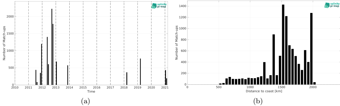
Figure 2: Number of match-ups between TSG (SAMOS) and SMOS SSS L4 v2 - Daily (BEC) SSS as a function of time (a) and as function of the distance to coast (b) over the SPURS 1 Pi-MEP region and for the full satellite product period.
