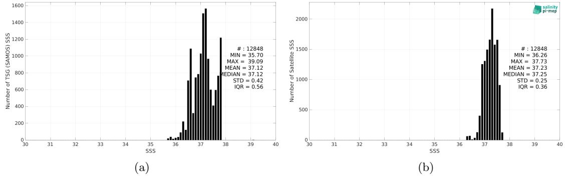
Figure 2: Histograms of SSS from TSG (SAMOS) (a) and SMOS SSS L4 v2 - Daily (BEC) (b) considering all match-up pairs per bins of 0.1 over the SPURS 1 Pi-MEP region and for the full satellite product period.
