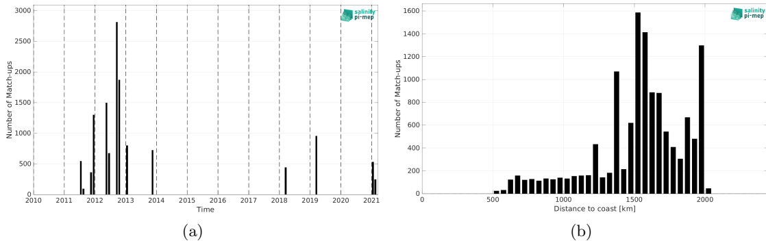
Figure 1: Number of match-ups between TSG (SAMOS) and SMOS SSS L4 v2 - Daily (BEC) SSS as a function of time (a) and as function of the distance to coast (b) over the SPURS 1 Pi-MEP region and for the full satellite product period.
