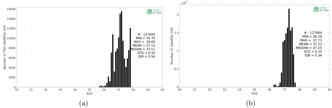
Figure 2: Histograms of SSS from TSG (SAMOS) (a) and SMOS SSS L4 v2 - Daily (BEC) (b) considering all match-up pairs per bins of 0.1 over the SPURS 1 Pi-MEP region and for the full satellite product period.
