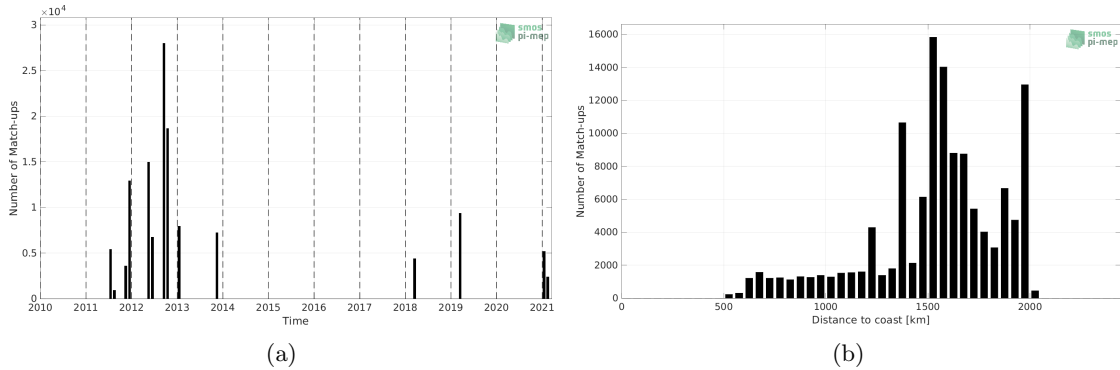
Figure 1: Number of match-ups between TSG (SAMOS) and SMOS SSS L4 v2 - Daily (BEC) SSS as a function of time (a) and as function of the distance to coast (b) over the SPURS 1 Pi-MEP region and for the full satellite product period.
