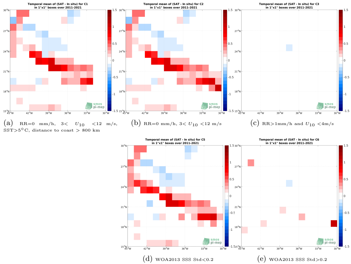
Figure 12: Temporal mean gridded over spatial boxes of size 1^\circ \times 1^\circ of \Delta SSS (SMOS SSS L4 v2 - Daily (BEC) - TSG (SAMOS)) for 5 different subdatasets corresponding to:RR=0 mm/h, 3 < U_{10} < 12 m/s, SST > 5^\circ\text{C} , distance to coast > 800 km (a), RR=0 mm/h, 3 < U_{10} < 12 m/s (b), RR > 1 mm/h and U_{10} < 4 m/s (c), WOA2013 SSS Std < 0.2 (d), WOA2013 SSS Std > 0.2 (e).
