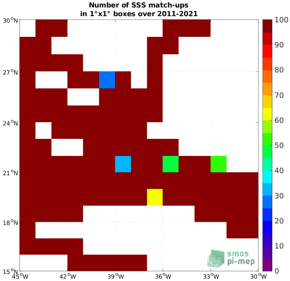
Figure 4: Number of SSS match-ups between TSG (SAMOS) SSS and the SMOS SSS L4 v2 - Daily (BEC) SSS product for the SPURS 1 Pi-MEP region over 1°x1° boxes and for the full satellite product period.
