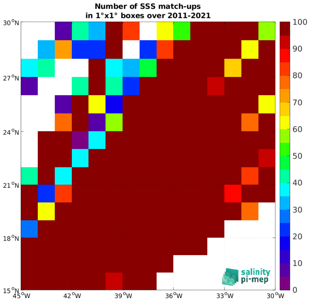
Figure 5: Number of SSS match-ups between TSG (LEGOS-DM) SSS and the SMOS SSS L4 v2 - Daily (BEC) SSS product for the SPURS 1 Pi-MEP region over 1^\circ \times 1^\circ boxes and for the full satellite product period.
