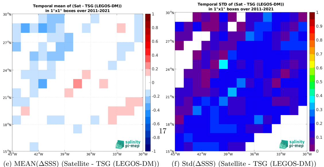
Figure 7: Temporal mean (left) and Std (right) of SSS from SMOS SSS L4 v2 - Daily (BEC) (top), TSG (LEGOS-DM) (middle), and of \Delta SSS (Satellite - TSG (LEGOS-DM)). Only match-up pairs are used to generate these maps.
