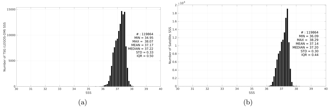
Figure 3: Histograms of SSS from TSG (LEGOS-DM) (a) and SMOS SSS L4 v2 - Daily (BEC) (b) considering all match-up pairs per bins of 0.1 over the SPURS 1 Pi-MEP region and for the full satellite product period.
