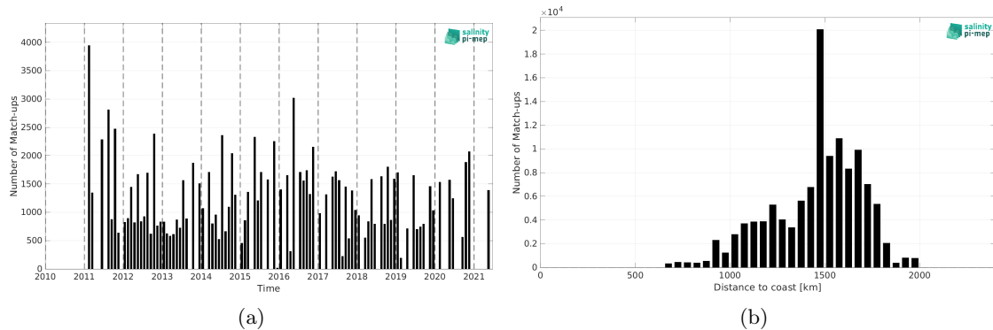
Figure 2: Number of match-ups between TSG (LEGOS-DM) and SMOS SSS L4 v2 - Daily (BEC) SSS as a function of time (a) and as function of the distance to coast (b) over the SPURS 1 Pi-MEP region and for the full satellite product period.
