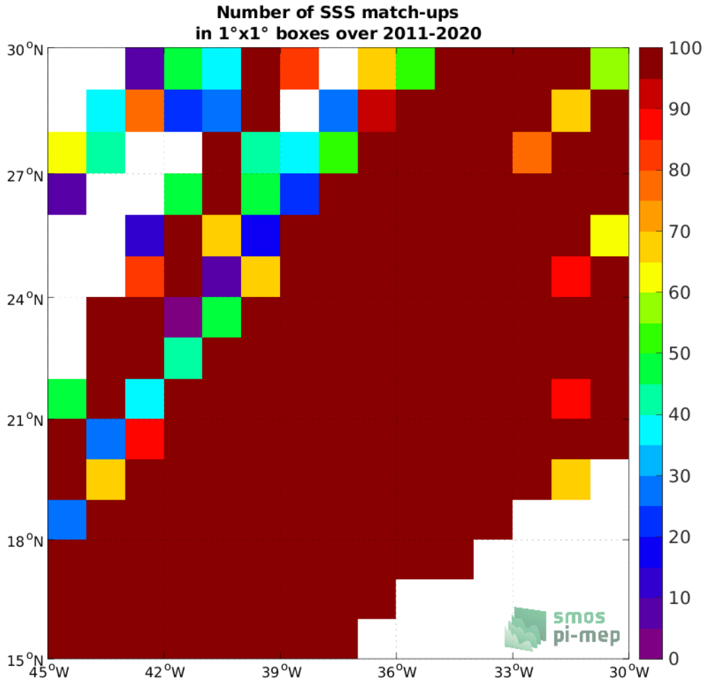
Figure 4: Number of SSS match-ups between TSG (LEGOS-DM) SSS and the SMOS SSS L4 v2 - Daily (BEC) SSS product for the SPURS 1 Pi-MEP region over 1^\circ \times 1^\circ boxes and for the full satellite product period.
