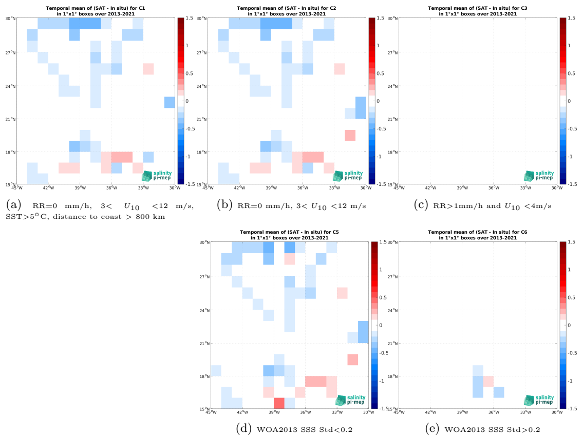
Figure 14: Temporal mean gridded over spatial boxes of size 1^\circ \times 1^\circ of \Delta SSS (SMOS SSS L4 v2 - Daily (BEC) - TSG (GOSUD-Sailing-ship)) for 5 different subdatasets corresponding to:RR=0 mm/h, 3 < U_{10} < 12 m/s, SST >5^\circ C, distance to coast > 800 km (a), RR=0 mm/h, 3 < U_{10} < 12 m/s (b), RR >1 mm/h and U_{10} < 4 m/s (c), WOA2013 SSS Std <0.2 (d), WOA2013 SSS Std >0.2 (e).
