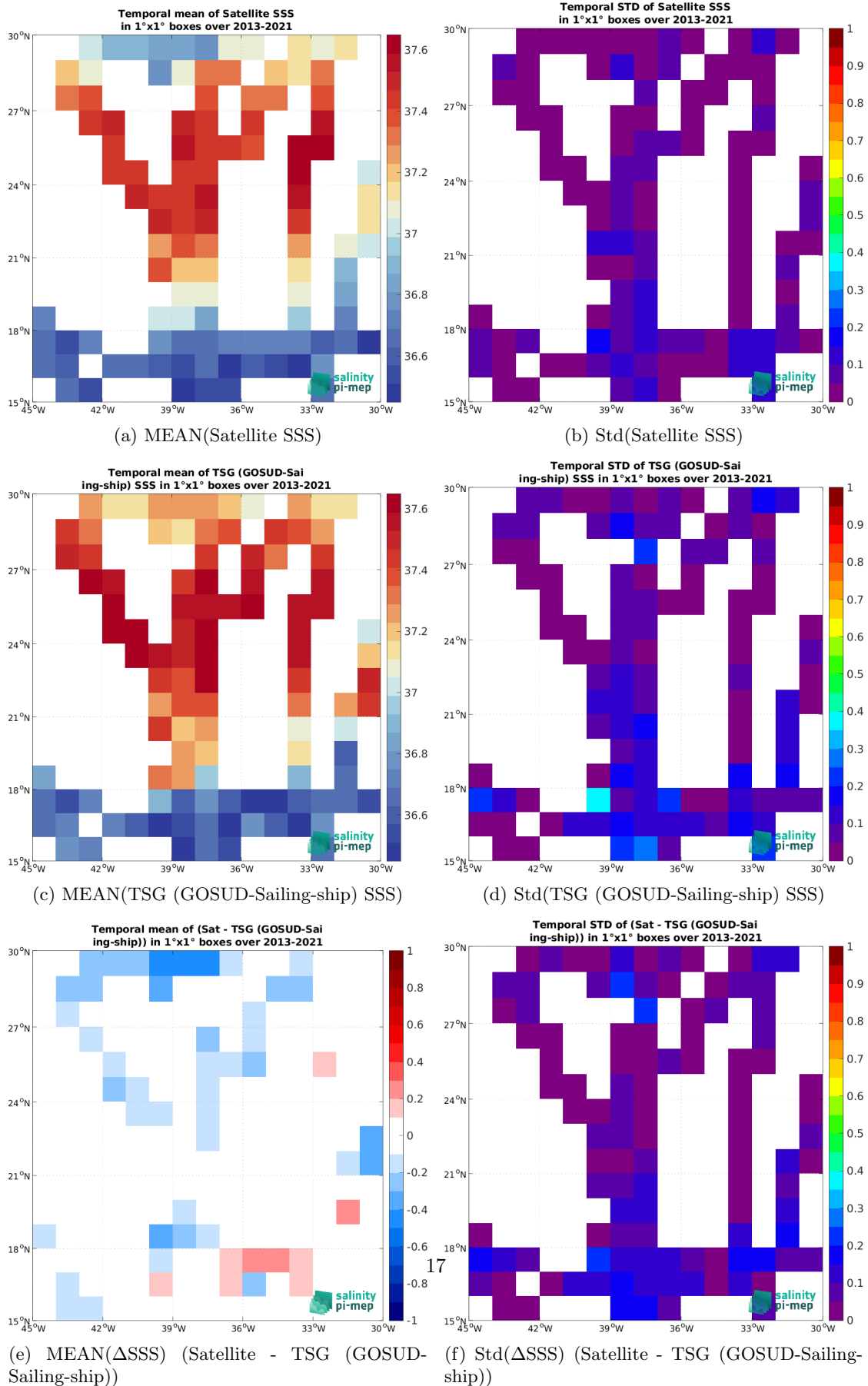
Figure 6: Temporal mean (left) and Std (right) of SSS from SMOS SSS L4 v2 - Daily (BEC) (top), TSG (GOSUD-Sailing-ship) (middle), and of \Delta SSS (Satellite - TSG (GOSUD-Sailing-ship)). Only match-up pairs are used to generate these maps.
