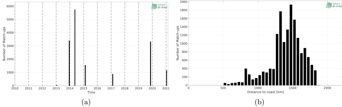
Figure 1: Number of match-ups between TSG (GOSUD-Sailing-ship) and SMOS SSS L4 v2 - Daily (BEC) SSS as a function of time (a) and as function of the distance to coast (b) over the SPURS 1 Pi-MEP region and for the full satellite product period.
