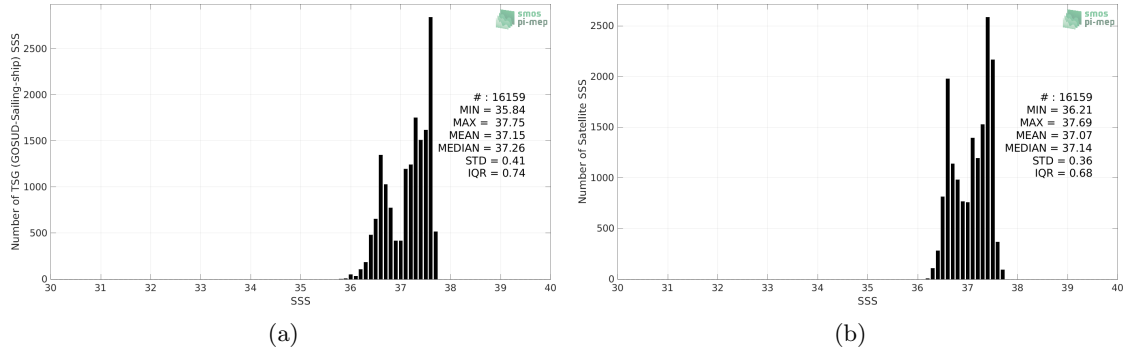
Figure 2: Histograms of SSS from TSG (GOSUD-Sailing-ship) (a) and SMOS SSS L4 v2 - Daily (BEC) (b) considering all match-up pairs per bins of 0.1 over the SPURS 1 Pi-MEP region and for the full satellite product period.
