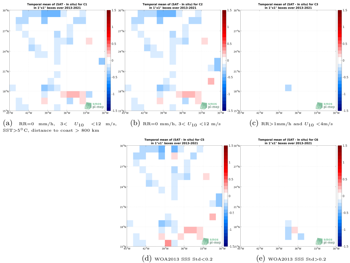
Figure 12: Temporal mean gridded over spatial boxes of size 1^\circ \times 1^\circ of \Delta SSS (SMOS SSS L4 v2 - Daily (BEC) - TSG (GOSUD-Sailing-ship)) for 5 different subdatasets corresponding to:RR=0 mm/h, 3 < U_{10} < 12 m/s, SST >5^\circ C, distance to coast > 800 km (a), RR=0 mm/h, 3 < U_{10} < 12 m/s (b), RR >1 mm/h and U_{10} < 4 m/s (c), WOA2013 SSS Std <0.2 (d), WOA2013 SSS Std >0.2 (e).
