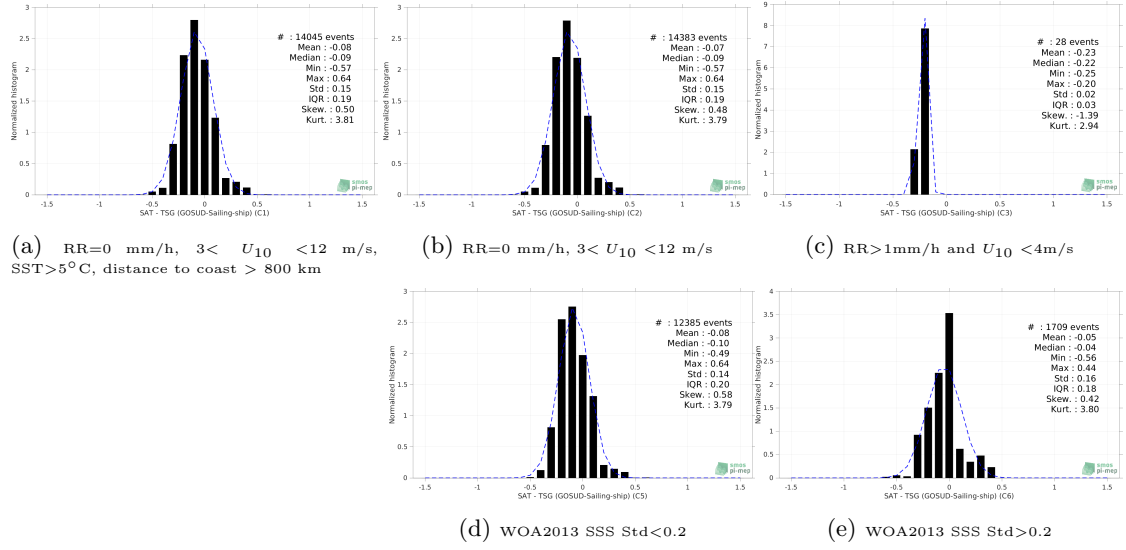
Figure 13: Normalized histogram of \Delta SSS (SMOS SSS L4 v2 - Daily (BEC) - TSG (GOSUD-Sailing-ship)) for 5 different subdatasets corresponding to: RR=0 mm/h, 3 < U_{10} < 12 m/s, SST>5°C, distance to coast > 800 km (a), RR=0 mm/h, 3 < U_{10} < 12 m/s (b), RR>1mm/h and U_{10} < 4 m/s (c), WOA2013 SSS Std<0.2 (d), WOA2013 SSS Std>0.2 (e).
