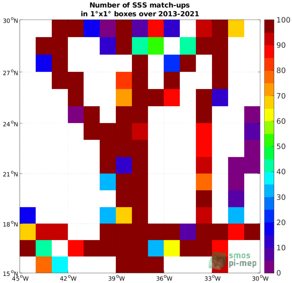
Figure 4: Number of SSS match-ups between TSG (GOSUD-Sailing-ship) SSS and the SMOS SSS L4 v2 - Daily (BEC) SSS product for the SPURS 1 Pi-MEP region over 1^\circ \times 1^\circ boxes and for the full satellite product period.
