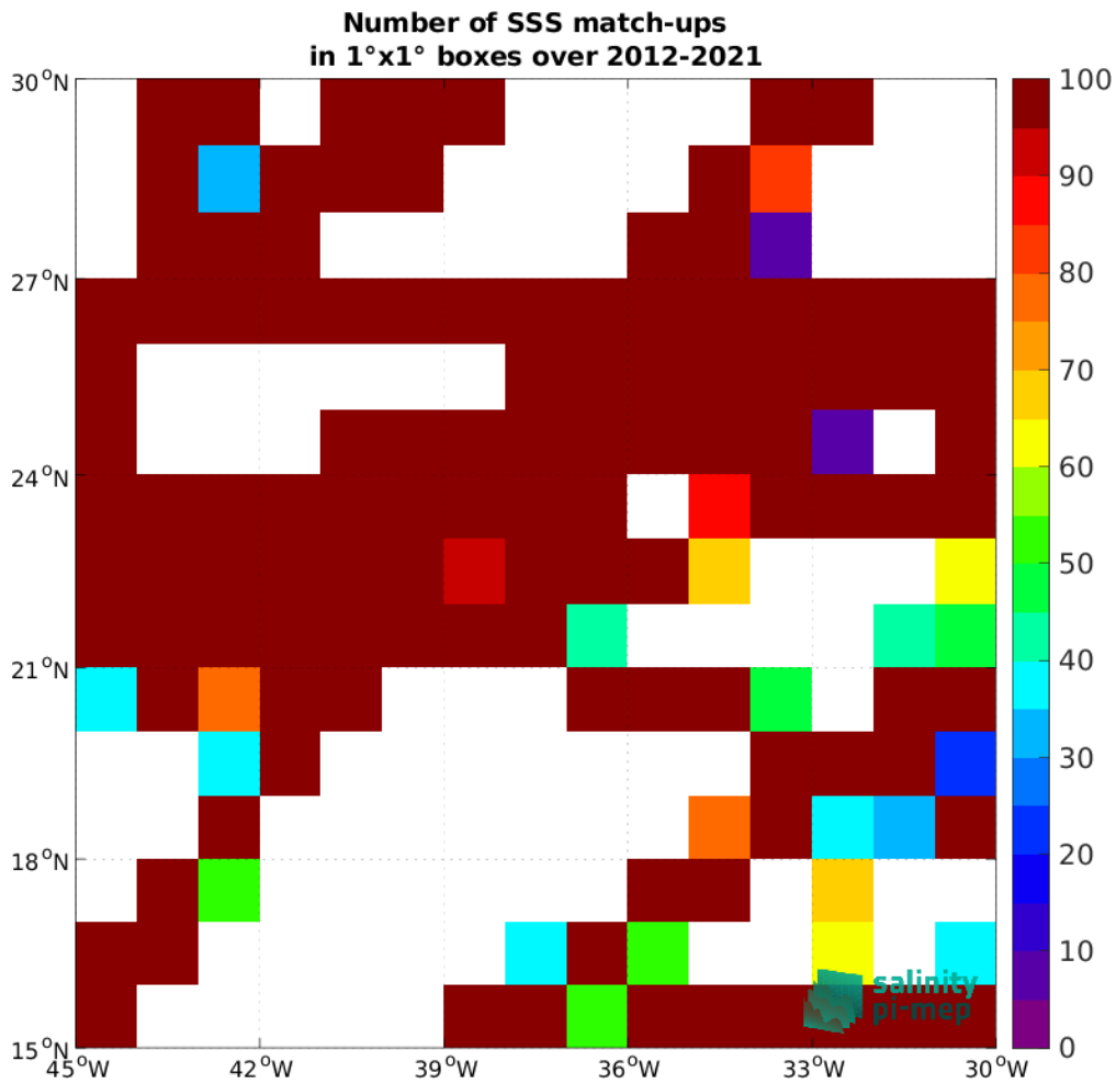
Figure 5: Number of SSS match-ups between TSG (GOSUD-Research-vessel) SSS and the SMOS SSS L4 v2 - Daily (BEC) SSS product for the SPURS 1 Pi-MEP region over 1°x1° boxes and for the full satellite product period.
