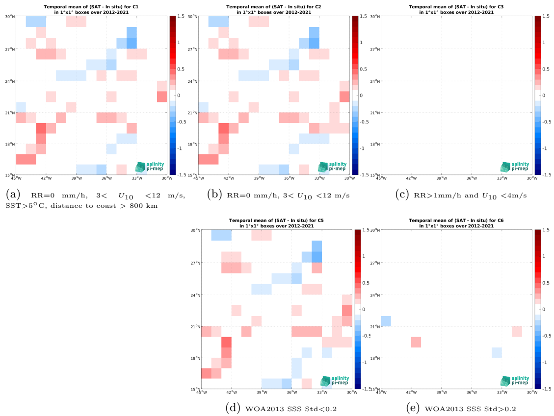
Figure 14: Temporal mean gridded over spatial boxes of size 1^\circ \times 1^\circ of \Delta\text{SSS} (SMOS SSS L4 v2 - Daily (BEC) - TSG (GOSUD-Research-vessel)) for 5 different subdatasets corresponding to:RR=0 mm/h, 3 < U_{10} < 12 m/s, SST>5°C, distance to coast > 800 km (a), RR=0 mm/h, 3 < U_{10} < 12 m/s (b), RR>1mm/h and U_{10} < 4 m/s (c), WOA2013 SSS Std<0.2 (d), WOA2013 SSS Std>0.2 (e).
