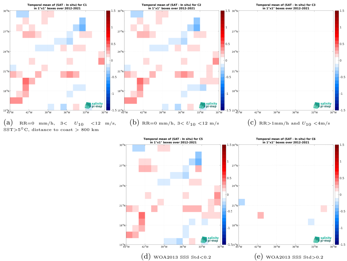
Figure 14: Temporal mean gridded over spatial boxes of size 1^\circ \times 1^\circ of \Delta SSS (SMOS SSS L4 v2 - Daily (BEC) - TSG (GOSUD-Research-vessel)) for 5 different subdatasets corresponding to:RR=0 mm/h, 3 < U_{10} < 12 m/s, SST >5^\circ C, distance to coast > 800 km (a), RR=0 mm/h, 3 < U_{10} < 12 m/s (b), RR >1 mm/h and U_{10} < 4 m/s (c), WOA2013 SSS Std <0.2 (d), WOA2013 SSS Std >0.2 (e).
