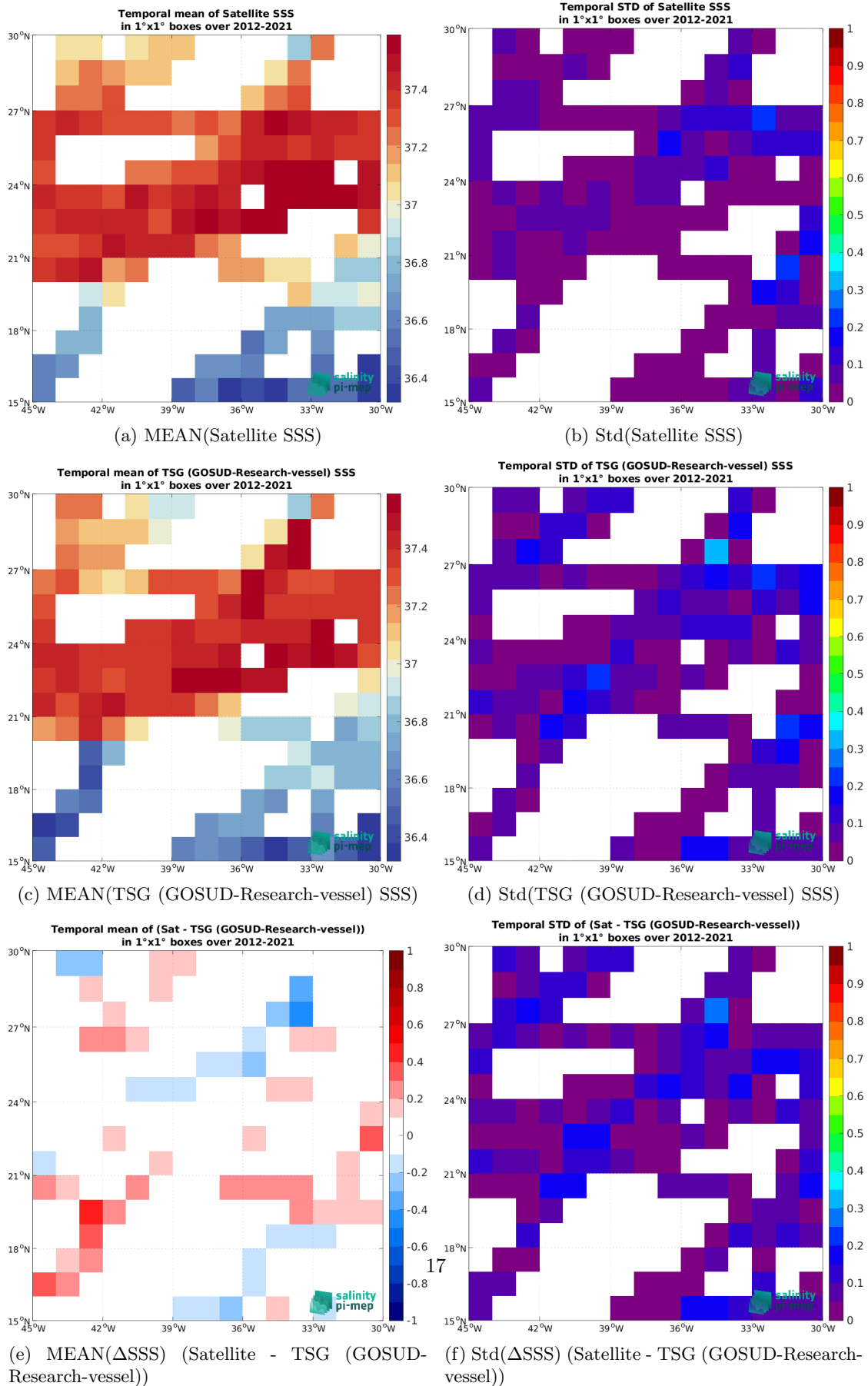
Figure 7: Temporal mean (left) and Std (right) of SSS from SMOS SSS L4 v2 - Daily (BEC) (top), TSG (GOSUD-Research-vessel) (middle), and of \Delta SSS (Satellite - TSG (GOSUD-Research-vessel)). Only match-up pairs are used to generate these maps.
