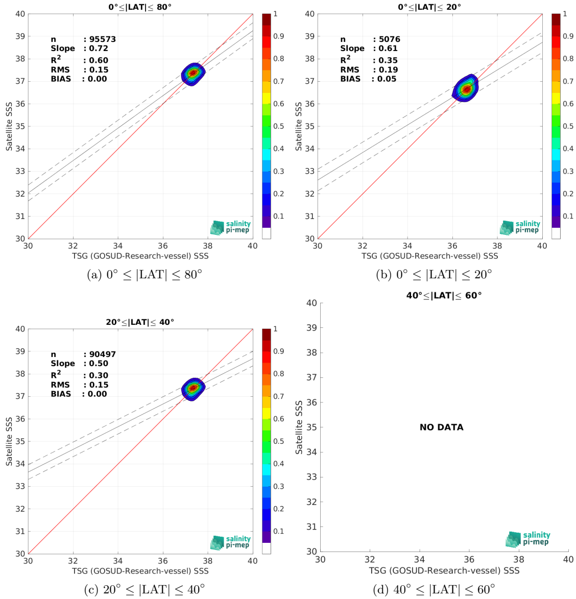
Figure 10: Contour maps of the concentration of SMOS SSS L4 v2 - Daily (BEC) SSS (y-axis) versus TSG (GOSUD-Research-vessel) SSS (x-axis) at match-up pairs for different latitude bands. For each plot, the red line shows x=y . The black thin and dashed lines indicate a linear fit through the data cloud and the \pm 95\% confidence levels, respectively. The number match-up pairs n , the slope and R^2 coefficient of the linear fit, the root mean square (RMS) and the mean bias between satellite and in situ data are indicated for each latitude band in each plots.
