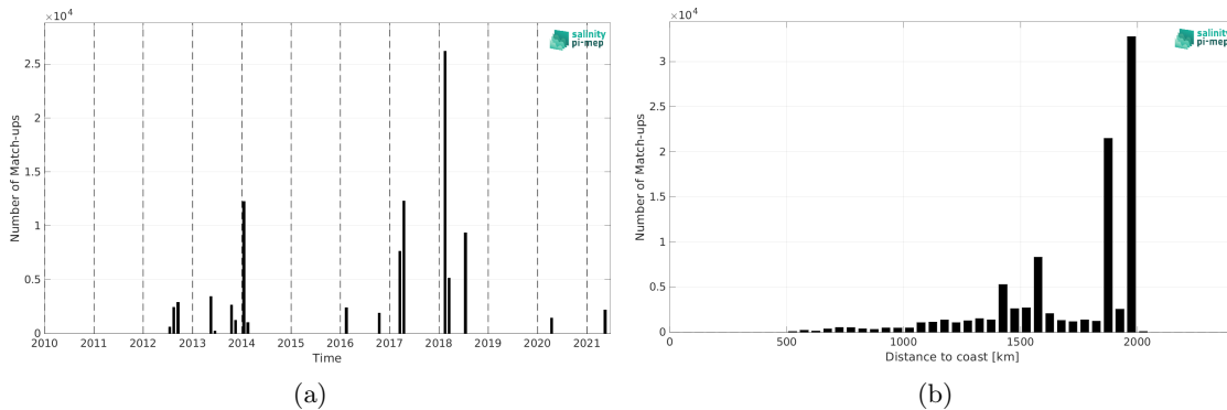
Figure 2: Number of match-ups between TSG (GOSUD-Research-vessel) and SMOS SSS L4 v2 - Daily (BEC) SSS as a function of time (a) and as function of the distance to coast (b) over the SPURS 1 Pi-MEP region and for the full satellite product period.
