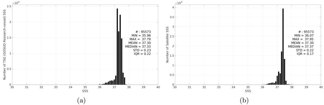
Figure 3: Histograms of SSS from TSG (GOSUD-Research-vessel) (a) and SMOS SSS L4 v2 - Daily (BEC) (b) considering all match-up pairs per bins of 0.1 over the SPURS 1 Pi-MEP region and for the full satellite product period.
