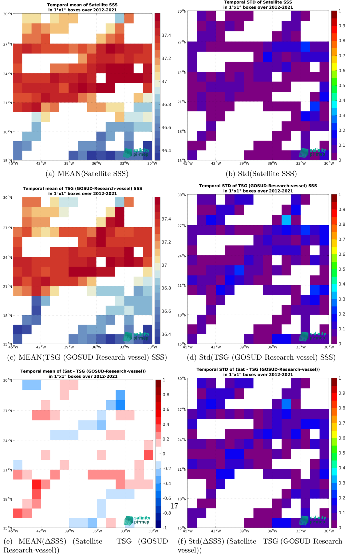
Figure 6: Temporal mean (left) and Std (right) of SSS from SMOS SSS L4 v2 - Daily (BEC) (top), TSG (GOSUD-Research-vessel) (middle), and of \Delta SSS (Satellite - TSG (GOSUD-Research-vessel)). Only match-up pairs are used to generate these maps.
