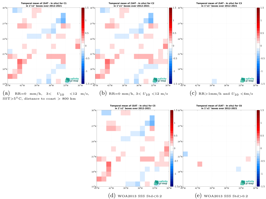
Figure 12: Temporal mean gridded over spatial boxes of size 1^\circ \times 1^\circ of \Delta SSS (SMOS SSS L4 v2 - Daily (BEC) - TSG (GOSUD-Research-vessel)) for 5 different subdatasets corresponding to:RR=0 mm/h, 3 < U_{10} < 12 m/s, SST>5°C, distance to coast > 800 km (a), RR=0 mm/h, 3 < U_{10} < 12 m/s (b), RR>1mm/h and U_{10} < 4 m/s (c), WOA2013 SSS Std<0.2 (d), WOA2013 SSS Std>0.2 (e).
