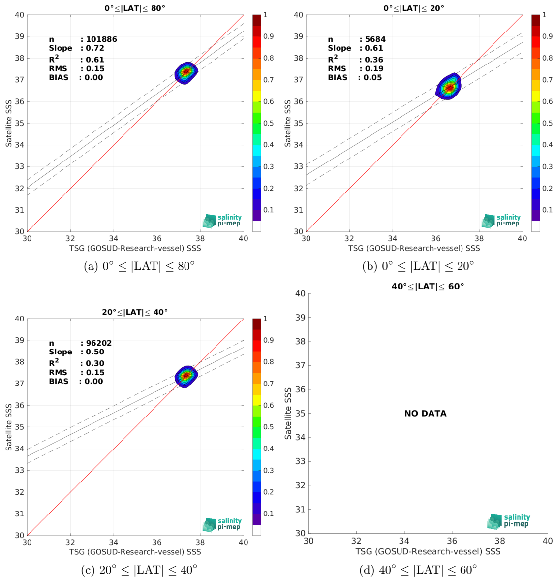
Figure 9: Contour maps of the concentration of SMOS SSS L4 v2 - Daily (BEC) SSS (y-axis) versus TSG (GOSUD-Research-vessel) SSS (x-axis) at match-up pairs for different latitude bands. For each plot, the red line shows x=y . The black thin and dashed lines indicate a linear fit through the data cloud and the \pm 95\% confidence levels, respectively. The number match-up pairs n , the slope and R^2 coefficient of the linear fit, the root mean square (RMS) and the mean bias between satellite and in situ data are indicated for each latitude band in each plots.
