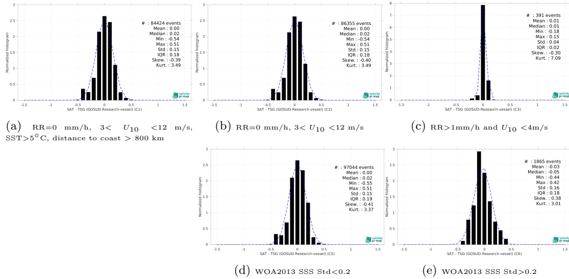
Figure 13: Normalized histogram of \Delta SSS (SMOS SSS L4 v2 - Daily (BEC) - TSG (GOSUD-Research-vessel)) for 5 different subdatasets corresponding to: RR=0 mm/h, 3 < U_{10} < 12 m/s, SST>5°C, distance to coast > 800 km (a), RR=0 mm/h, 3 < U_{10} < 12 m/s (b), RR>1mm/h and U_{10} < 4 m/s (c), WOA2013 SSS Std<0.2 (d), WOA2013 SSS Std>0.2 (e).
