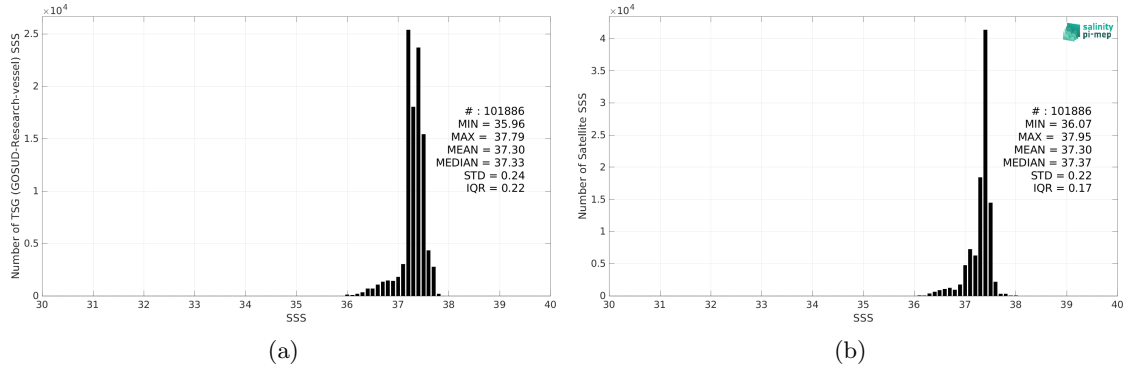
Figure 2: Histograms of SSS from TSG (GOSUD-Research-vessel) (a) and SMOS SSS L4 v2 - Daily (BEC) (b) considering all match-up pairs per bins of 0.1 over the SPURS 1 Pi-MEP region and for the full satellite product period.
