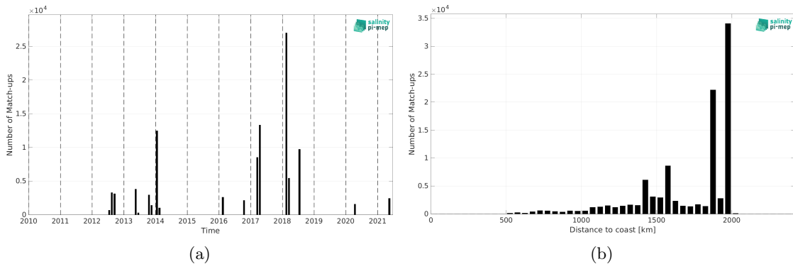
Figure 1: Number of match-ups between TSG (GOSUD-Research-vessel) and SMOS SSS L4 v2 - Daily (BEC) SSS as a function of time (a) and as function of the distance to coast (b) over the SPURS 1 Pi-MEP region and for the full satellite product period.
