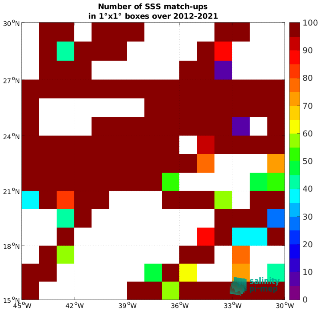
Figure 4: Number of SSS match-ups between TSG (GOSUD-Research-vessel) SSS and the SMOS SSS L4 v2 - Daily (BEC) SSS product for the SPURS 1 Pi-MEP region over 1°x1° boxes and for the full satellite product period.
