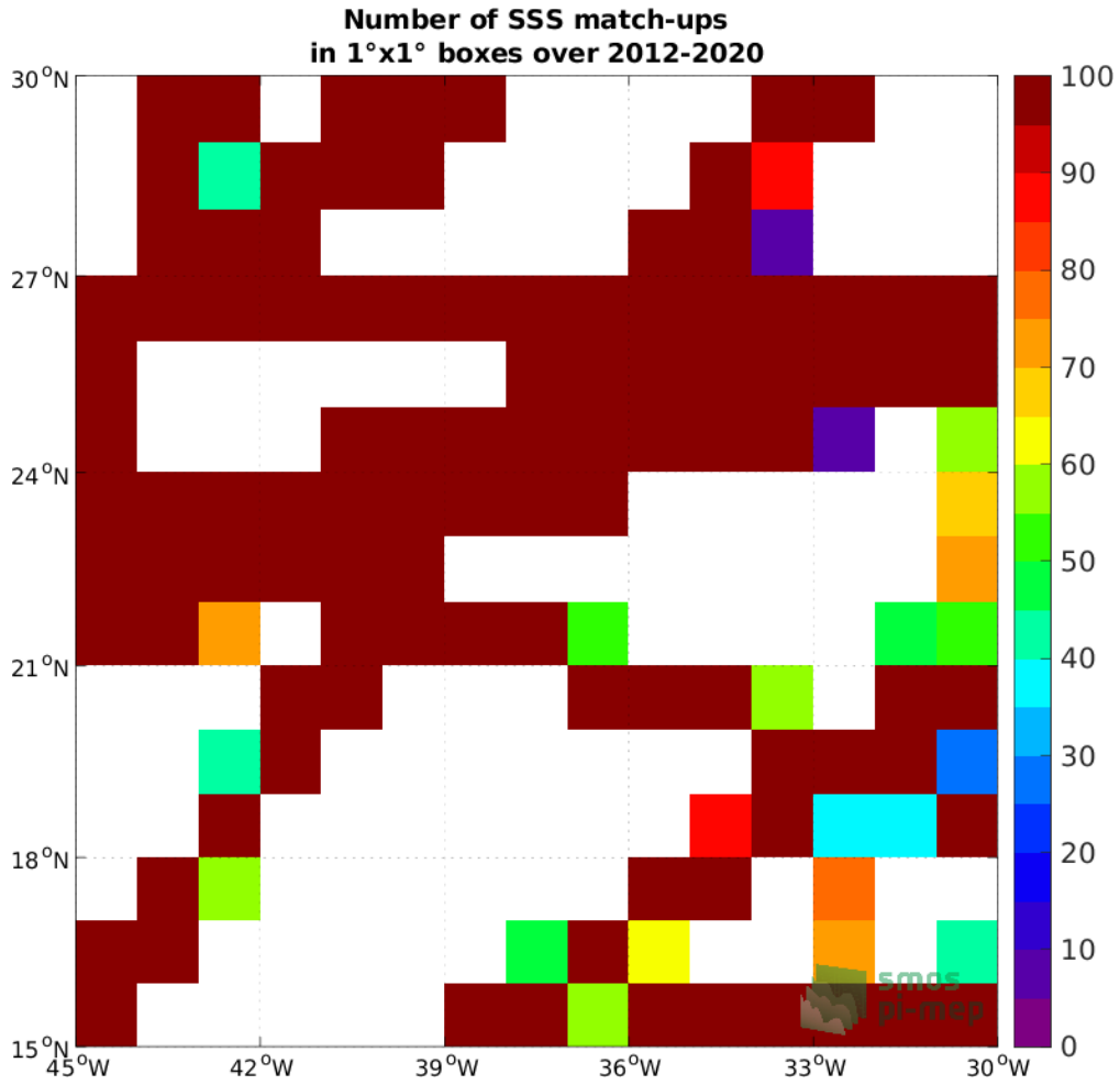
Figure 4: Number of SSS match-ups between TSG (GOSUD-Research-vessel) SSS and the SMOS SSS L4 v2 - Daily (BEC) SSS product for the SPURS 1 Pi-MEP region over 1^\circ \times 1^\circ boxes and for the full satellite product period.
