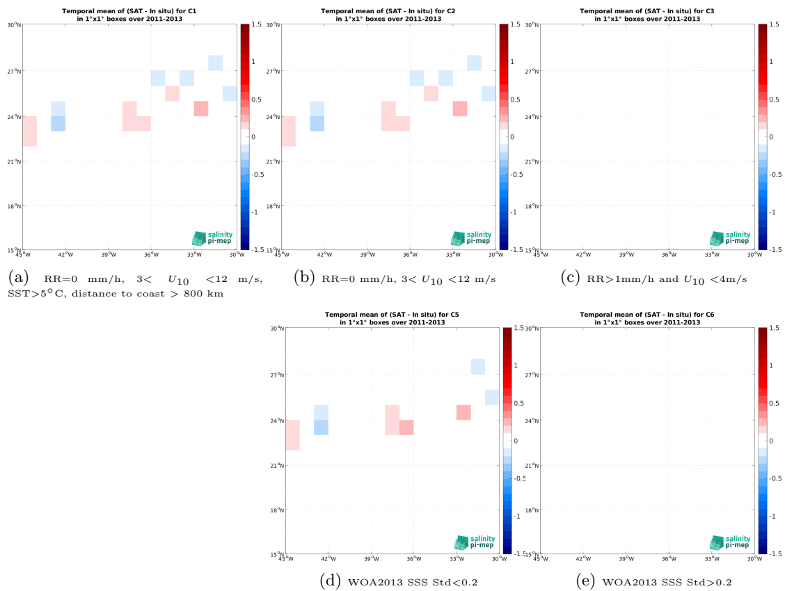
Figure 14: Temporal mean gridded over spatial boxes of size 1^\circ \times 1^\circ of \Delta\text{SSS} (SMOS SSS L4 v2 - Daily (BEC) - TSG (CSIC-UTM)) for 5 different subdatasets corresponding to: RR=0 mm/h, 3 < U_{10} < 12 m/s, SST > 5°C, distance to coast > 800 km (a), RR=0 mm/h, 3 < U_{10} < 12 m/s (b), RR > 1mm/h and U_{10} < 4 m/s (c), WOA2013 SSS Std < 0.2 (d), WOA2013 SSS Std > 0.2 (e).
