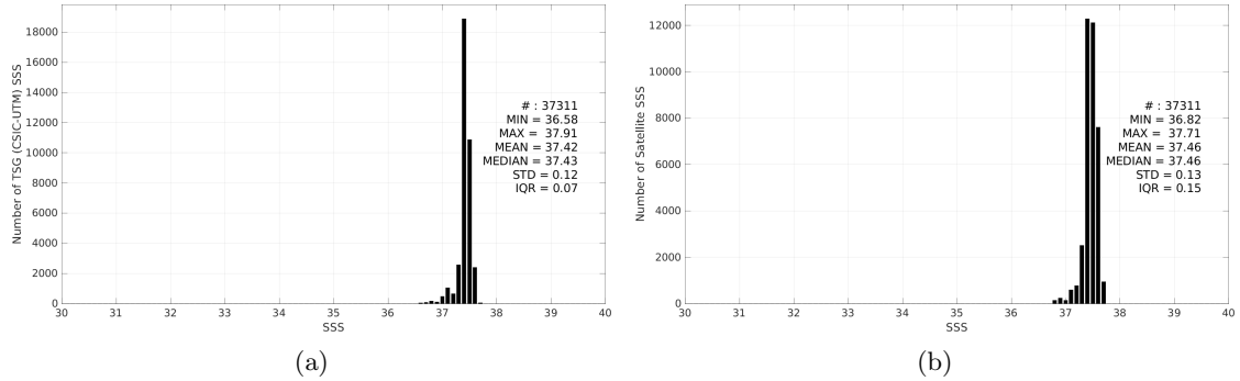
Figure 3: Histograms of SSS from TSG (CSIC-UTM) (a) and SMOS SSS L4 v2 - Daily (BEC) (b) considering all match-up pairs per bins of 0.1 over the SPURS 1 Pi-MEP region and for the full satellite product period.
