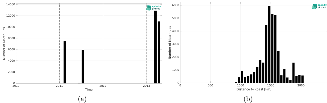
Figure 2: Number of match-ups between TSG (CSIC-UTM) and SMOS SSS L4 v2 - Daily (BEC) SSS as a function of time (a) and as function of the distance to coast (b) over the SPURS 1 Pi-MEP region and for the full satellite product period.
