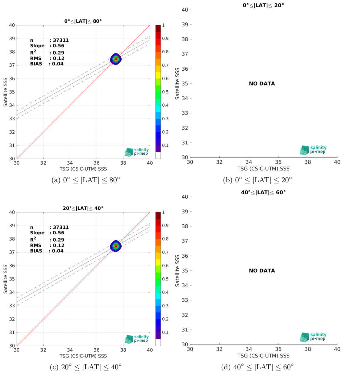
Figure 10: Contour maps of the concentration of SMOS SSS L4 v2 - Daily (BEC) SSS (y-axis) versus TSG (CSIC-UTM) SSS (x-axis) at match-up pairs for different latitude bands. For each plot, the red line shows x=y . The black thin and dashed lines indicate a linear fit through the data cloud and the \pm 95\% confidence levels, respectively. The number match-up pairs n , the slope and R^2 coefficient of the linear fit, the root mean square (RMS) and the mean bias between satellite and in situ data are indicated for each latitude band in each plots.
