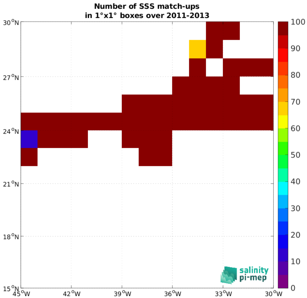
Figure 5: Number of SSS match-ups between TSG (CSIC-UTM) SSS and the SMOS SSS L4 v2 - Daily (BEC) SSS product for the SPURS 1 Pi-MEP region over 1^\circ \times 1^\circ boxes and for the full satellite product period.
