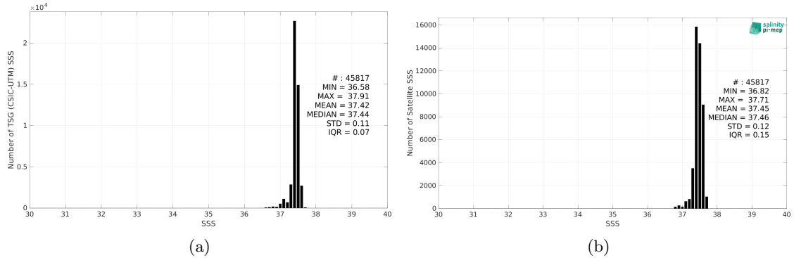
Figure 2: Histograms of SSS from TSG (CSIC-UTM) (a) and SMOS SSS L4 v2 - Daily (BEC) (b) considering all match-up pairs per bins of 0.1 over the SPURS 1 Pi-MEP region and for the full satellite product period.
