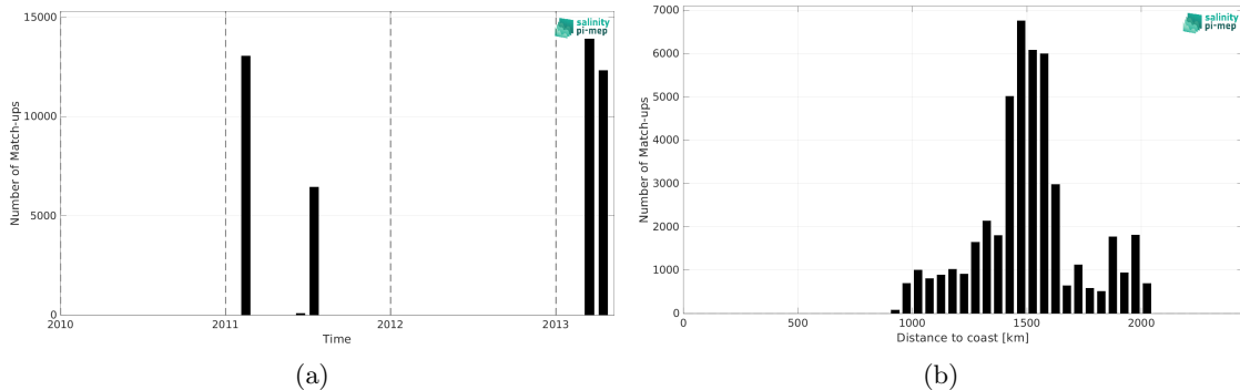
Figure 1: Number of match-ups between TSG (CSIC-UTM) and SMOS SSS L4 v2 - Daily (BEC) SSS as a function of time (a) and as function of the distance to coast (b) over the SPURS 1 Pi-MEP region and for the full satellite product period.
