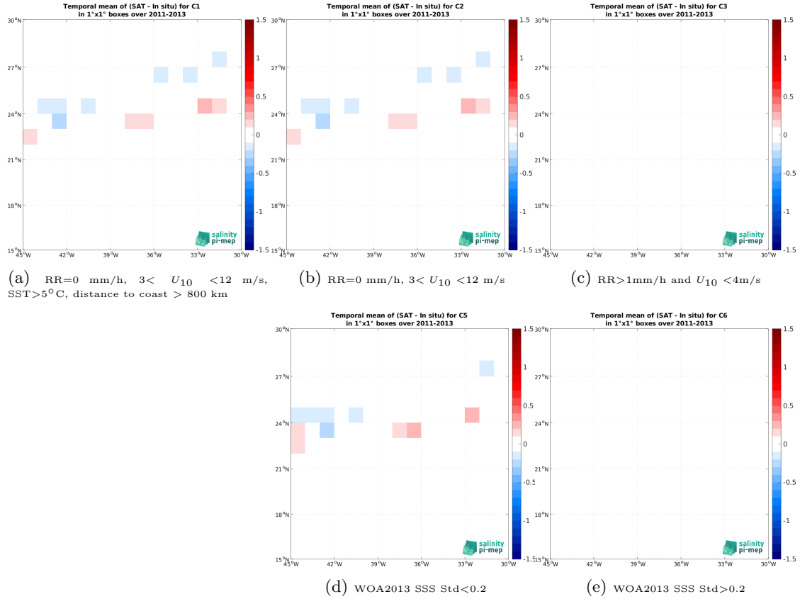
Figure 12: Temporal mean gridded over spatial boxes of size 1^{\circ}\times 1^{\circ} of \Delta\text{SSS} (SMOS SSS L4 v2 - Daily (BEC) - TSG (CSIC-UTM)) for 5 different subdatasets corresponding to:RR=0 mm/h, 3 < U_{10} < 12 m/s, \text{SST}>5^{\circ}\text{C} , distance to coast > 800 km (a), RR=0 mm/h, 3 < U_{10} < 12 m/s (b), RR >1\text{mm/h} and U_{10} < 4\text{m/s} (c), WOA2013 SSS Std <0.2 (d), WOA2013 SSS Std >0.2 (e).
