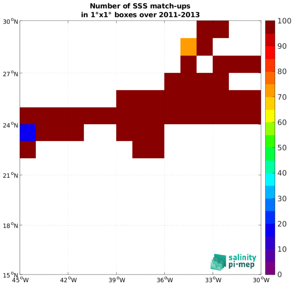
Figure 4: Number of SSS match-ups between TSG (CSIC-UTM) SSS and the SMOS SSS L4 v2 - Daily (BEC) SSS product for the SPURS 1 Pi-MEP region over 1^\circ \times 1^\circ boxes and for the full satellite product period.
