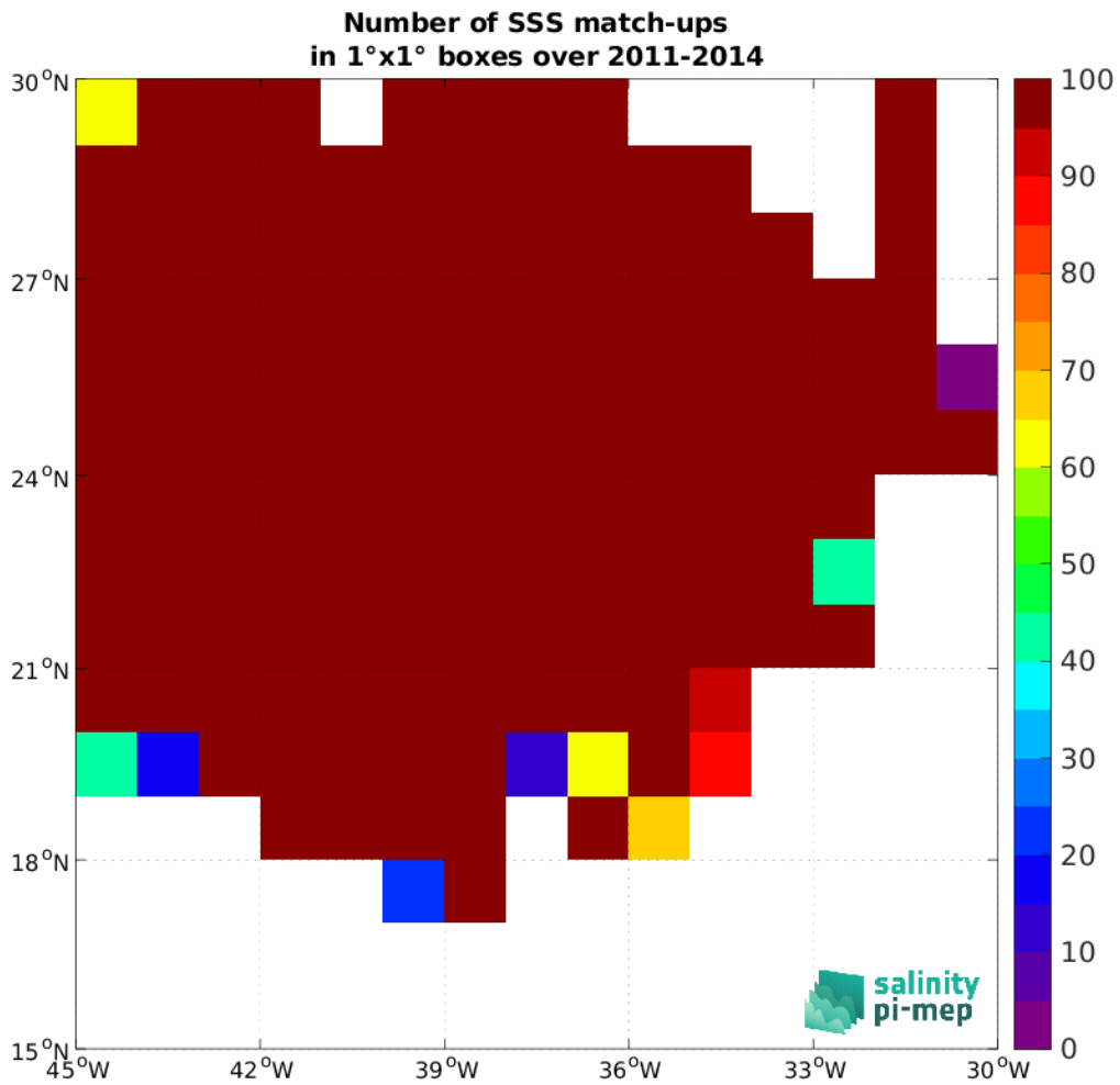
Figure 4: Number of SSS match-ups between Surface drifters SSS and the SMOS SSS L4 v2 - Daily (BEC) SSS product for the SPURS 1 Pi-MEP region over 1°x1° boxes and for the full satellite product period.
