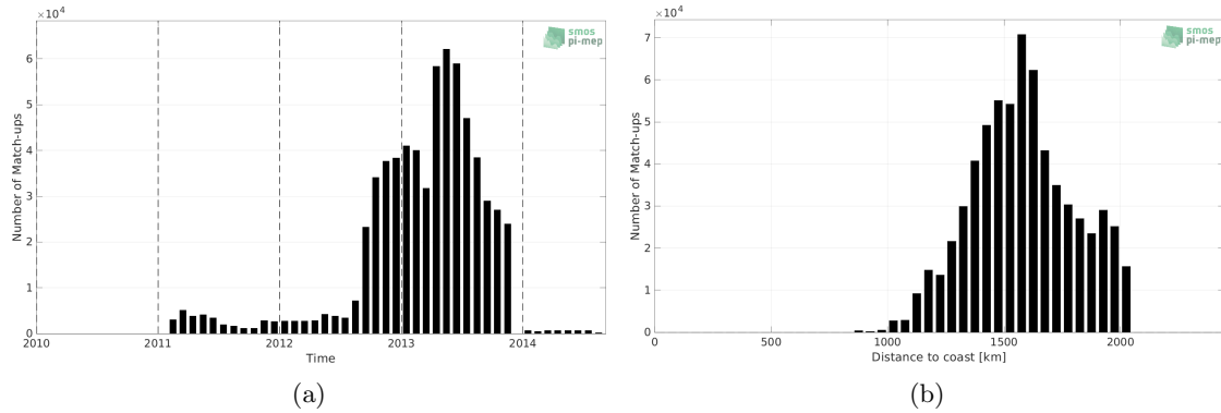
Figure 1: Number of match-ups between Surface drifters and SMOS SSS L4 v2 - Daily (BEC) SSS as a function of time (a) and as function of the distance to coast (b) over the SPURS 1 Pi-MEP region and for the full satellite product period.
