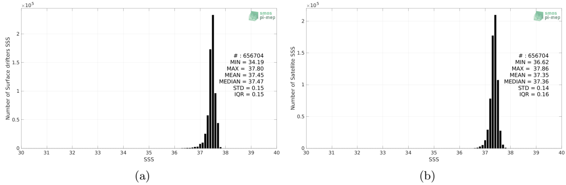
Figure 2: Histograms of SSS from Surface drifters (a) and SMOS SSS L4 v2 - Daily (BEC) (b) considering all match-up pairs per bins of 0.1 over the SPURS 1 Pi-MEP region and for the full satellite product period.
