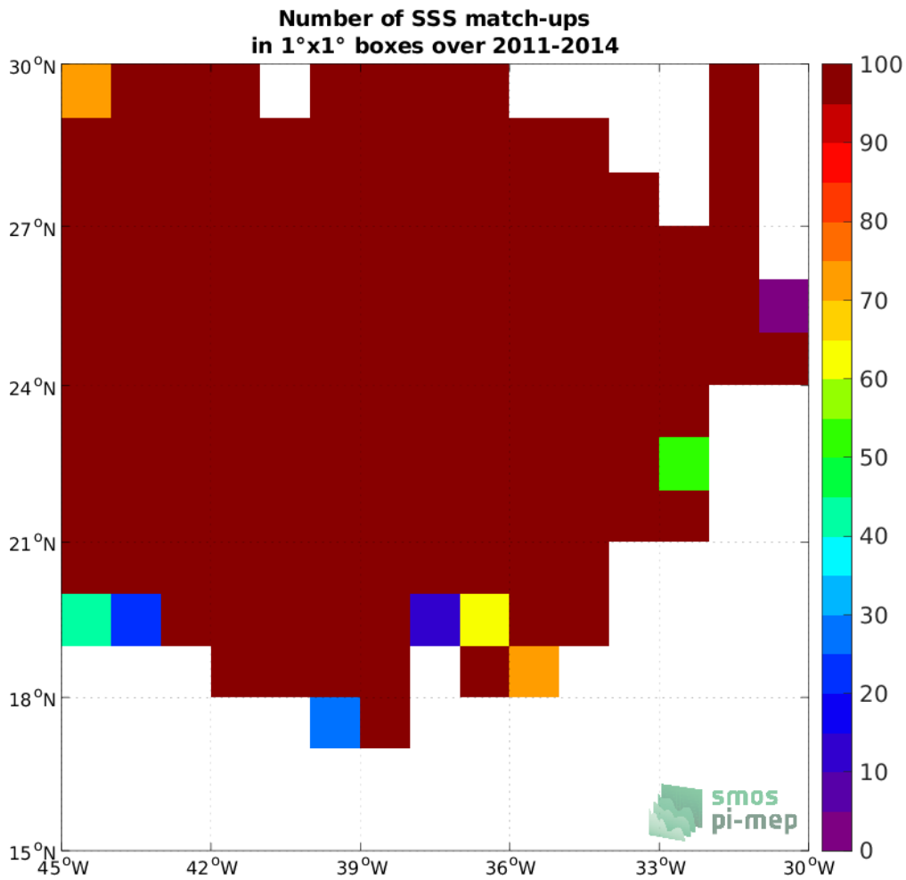
Figure 3: Number of SSS match-ups between Surface drifters SSS and the SMOS SSS L4 v2 - Daily (BEC) SSS product for the SPURS 1 Pi-MEP region over 1°x1° boxes and for the full satellite product period.
