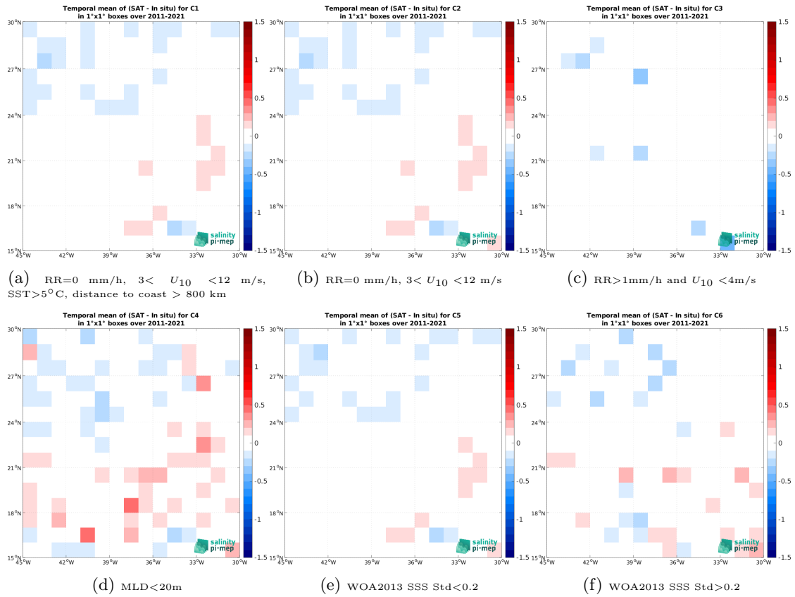
Figure 14: Temporal mean gridded over spatial boxes of size 1^\circ \times 1^\circ of \Delta SSS (SMOS SSS L4 v2 - Daily (BEC) - Argo) for 6 different subdatasets corresponding to:RR=0 mm/h, 3 < U_{10} < 12 m/s, SST >5^\circ\text{C} , distance to coast > 800 km (a), RR=0 mm/h, 3 < U_{10} < 12 m/s (b), RR >1 mm/h and U_{10} < 4 m/s (c),MLD <20 m (d),WOA2013 SSS Std <0.2 (e),WOA2013 SSS Std >0.2 (f).
