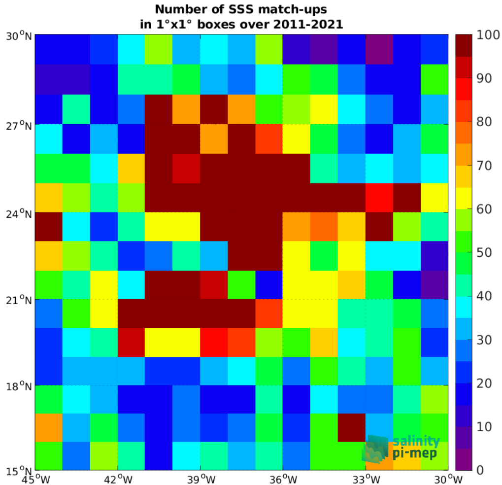
Figure 5: Number of SSS match-ups between Argo SSS and the SMOS SSS L4 v2 - Daily (BEC) SSS product for the SPURS 1 Pi-MEP region over 1^\circ \times 1^\circ boxes and for the full satellite product period.
