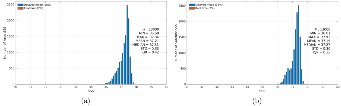
Figure 3: Histograms of SSS from Argo (a) and SMOS SSS L4 v2 - Daily (BEC) (b) considering all match-up pairs per bins of 0.1 over the SPURS 1 Pi-MEP region and for the full satellite product period.
