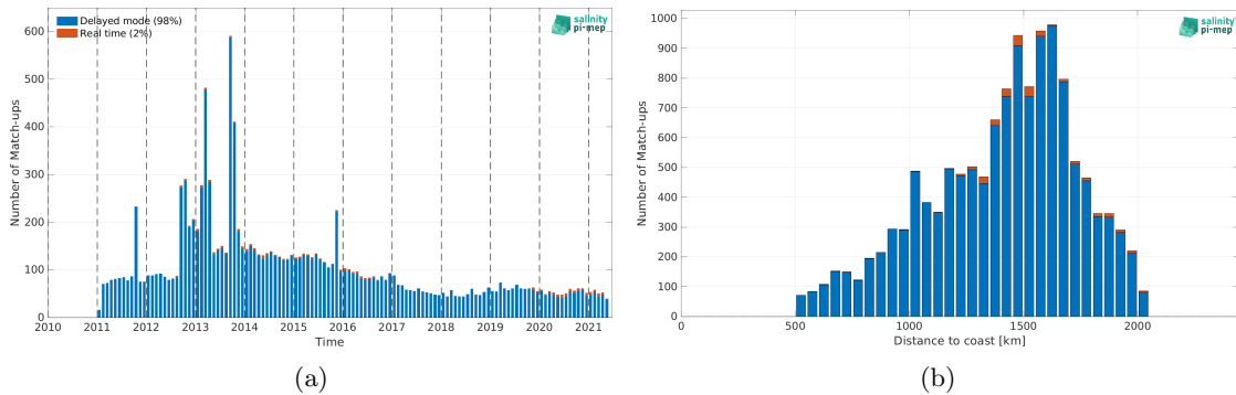
Figure 2: Number of match-ups between Argo and SMOS SSS L4 v2 - Daily (BEC) SSS as a function of time (a) and as function of the distance to coast (b) over the SPURS 1 Pi-MEP region and for the full satellite product period.
