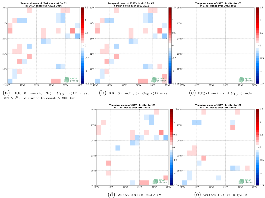
Figure 12: Temporal mean gridded over spatial boxes of size 1^\circ \times 1^\circ of \Delta\text{SSS} (SMOS SSS L3 v3 Monthly (ICDC) - TSG (GOSUD-Research-vessel)) for 5 different subdatasets corresponding to:RR=0 mm/h, 3 < U_{10} < 12 m/s, SST>5°C, distance to coast > 800 km (a), RR=0 mm/h, 3 < U_{10} < 12 m/s (b), RR>1mm/h and U_{10} < 4 m/s (c), WOA2013 SSS Std<0.2 (d), WOA2013 SSS Std>0.2 (e).
