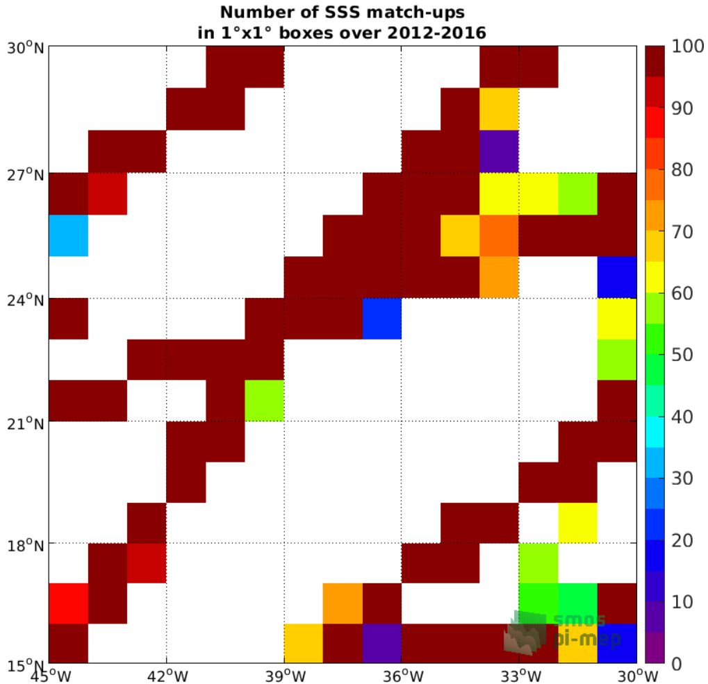
Figure 4: Number of SSS match-ups between TSG (GOSUD-Research-vessel) SSS and the SMOS SSS L3 v3 Monthly (ICDC) SSS product for the SPURS 1 Pi-MEP region over 1^{\circ} \times 1^{\circ} boxes and for the full satellite product period.
