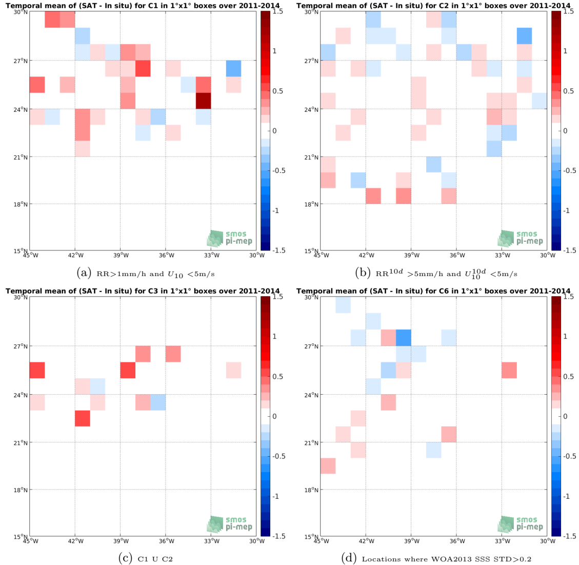
Figure 11: Temporal mean gridded over spatial boxes of size 1^\circ \times 1^\circ of \Delta SSS (SMOS-L3-ICDC-V3-MONTHLY-0.5DEG - Surface drifters) for 4 different subdatasets corresponding to: RR > 1\text{mm/h} and U_{10} < 5\text{m/s} (a), RR^{10d} > 5\text{mm/h} and U_{10}^{10d} < 5\text{m/s} (b), C1 U C2 (c), Locations where WOA2013 SSS STD > 0.2 (d).
