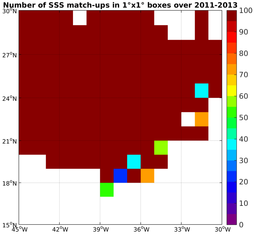
Figure 3: Number of SSS match-ups between Surface drifters SSS and the SMOS-L3-ICDC-V3-MONTHLY-0.5DEG SSS product for the SPURS 1 Pi-MEP region over 1°x1° boxes and for the full satellite product period.
