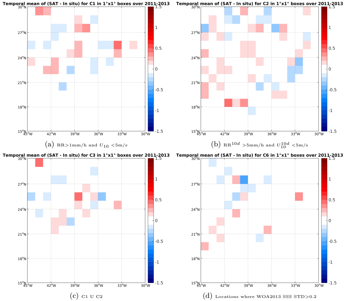
Figure 11: Temporal mean gridded over spatial boxes of size 1°x1° of \Delta SSS (SMOS-L3-ICDC-V3-MONTHLY-0.5DEG - Surface drifters) for 4 different subdatasets corresponding to:RR>1mm/h and U_{10} < 5\text{m/s} (a), RR^{10d} > 5\text{mm/h} and U_{10}^{10d} < 5\text{m/s} (b), C1 U C2 (c),Locations where WOA2013 SSS STD>0.2 (d).
