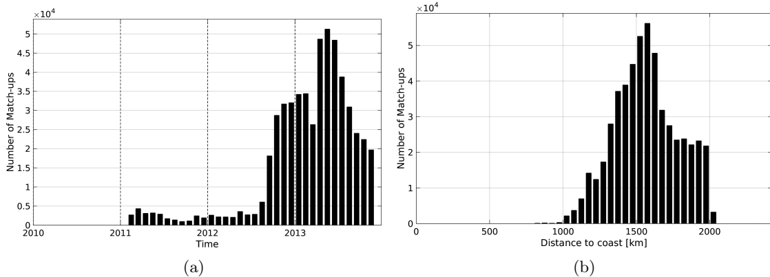
Figure 1: Number of match-ups between Surface drifters and SMOS-L3-ICDC-V3-MONTHLY-0.5DEG SSS as a function of time (a) and as function of the distance to coast (b) over the SPURS 1 Pi-MEP region and for the full satellite product period.
