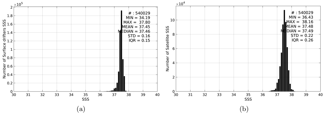
Figure 2: Histograms of SSS from Surface drifters (a) and SMOS-L3-ICDC-V3-MONTHLY-0.5DEG (b) considering all match-up pairs per bins of 0.1 over the SPURS 1 Pi-MEP region and for the full satellite product period.
