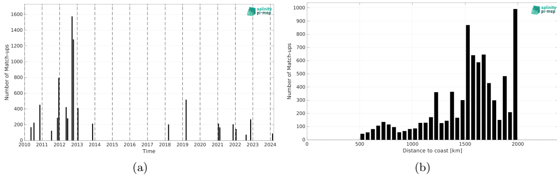
Figure 2: Number of match-ups between TSG (SAMOS) and SMOS SSS L2Q v331 - With FLAG (CMEMS-CATDS-CPDC) SSS as a function of time (a) and as function of the distance to coast (b) over the SPURS 1 Pi-MEP region and for the full satellite product period.
