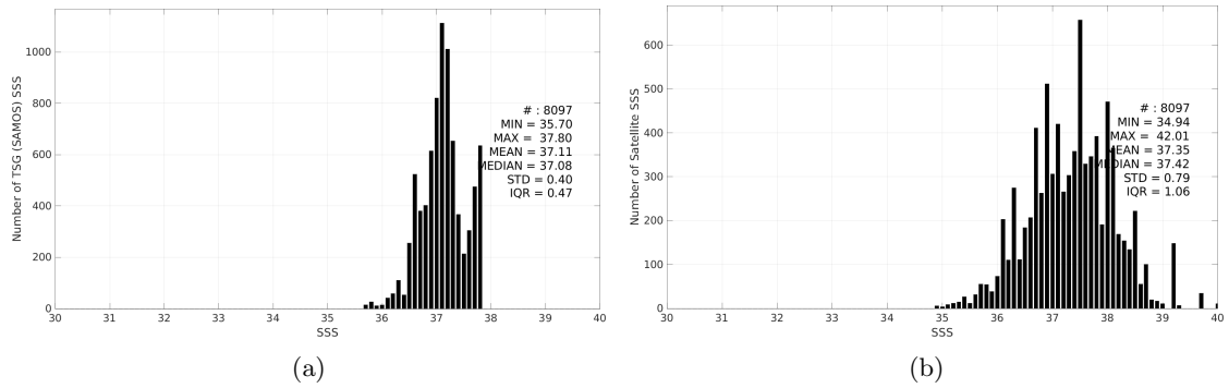
Figure 3: Histograms of SSS from TSG (SAMOS) (a) and SMOS SSS L2Q v331 - With FLAG (CMEMS-CATDS-CPDC) (b) considering all match-up pairs per bins of 0.1 over the SPURS 1 Pi-MEP region and for the full satellite product period.
