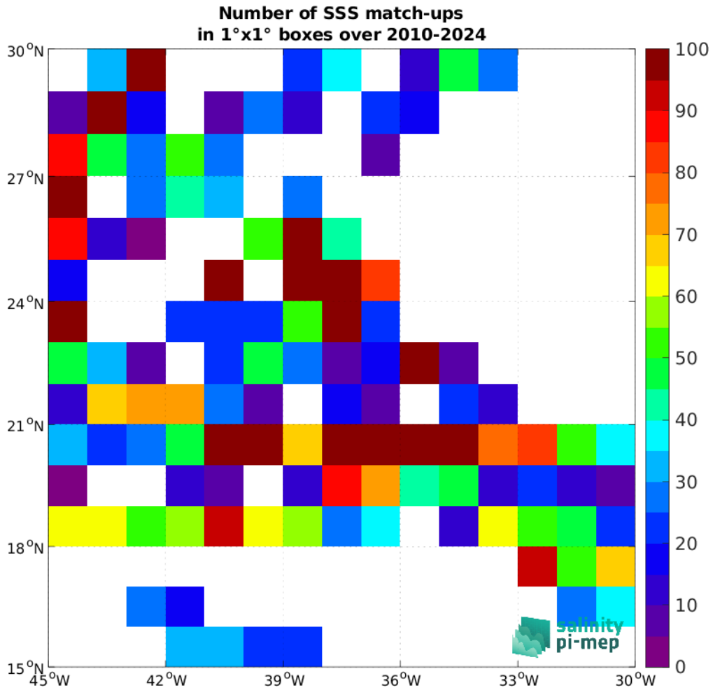
Figure 5: Number of SSS match-ups between TSG (SAMOS) SSS and the SMOS SSS L2Q v331 - With FLAG (CMEMS-CATDS-CPDC) SSS product for the SPURS 1 Pi-MEP region over 1^\circ \times 1^\circ boxes and for the full satellite product period.
