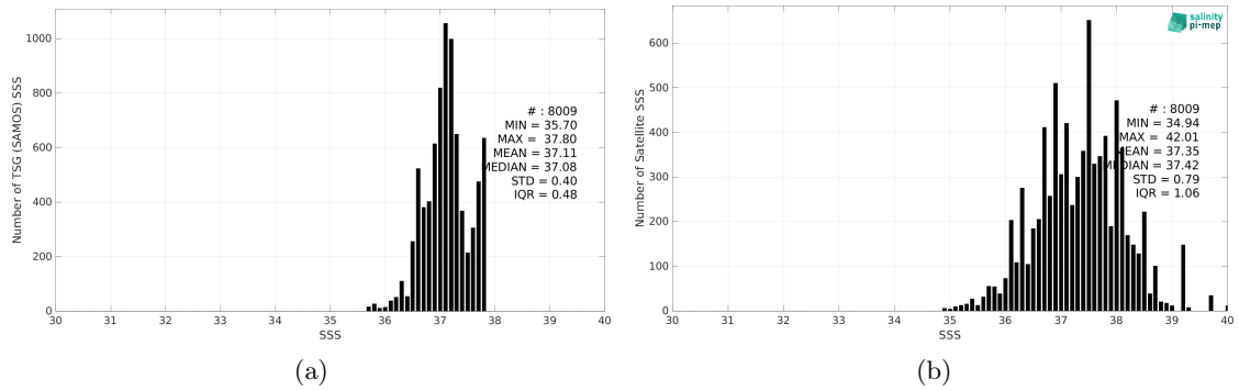
Figure 2: Histograms of SSS from TSG (SAMOS) (a) and SMOS SSS L2Q v331 - With FLAG (CMEMS-CATDS-CPDC) (b) considering all match-up pairs per bins of 0.1 over the SPURS 1 Pi-MEP region and for the full satellite product period.
