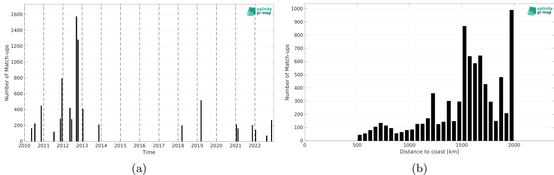
Figure 1: Number of match-ups between TSG (SAMOS) and SMOS SSS L2Q v331 - With FLAG (CMEMS-CATDS-CPDC) SSS as a function of time (a) and as function of the distance to coast (b) over the SPURS 1 Pi-MEP region and for the full satellite product period.
