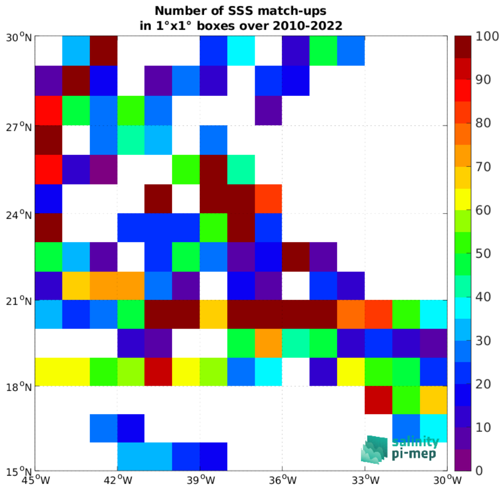
Figure 4: Number of SSS match-ups between TSG (SAMOS) SSS and the SMOS SSS L2Q v331 - With FLAG (CMEMS-CATDS-CPDC) SSS product for the SPURS 1 Pi-MEP region over 1°x1° boxes and for the full satellite product period.
