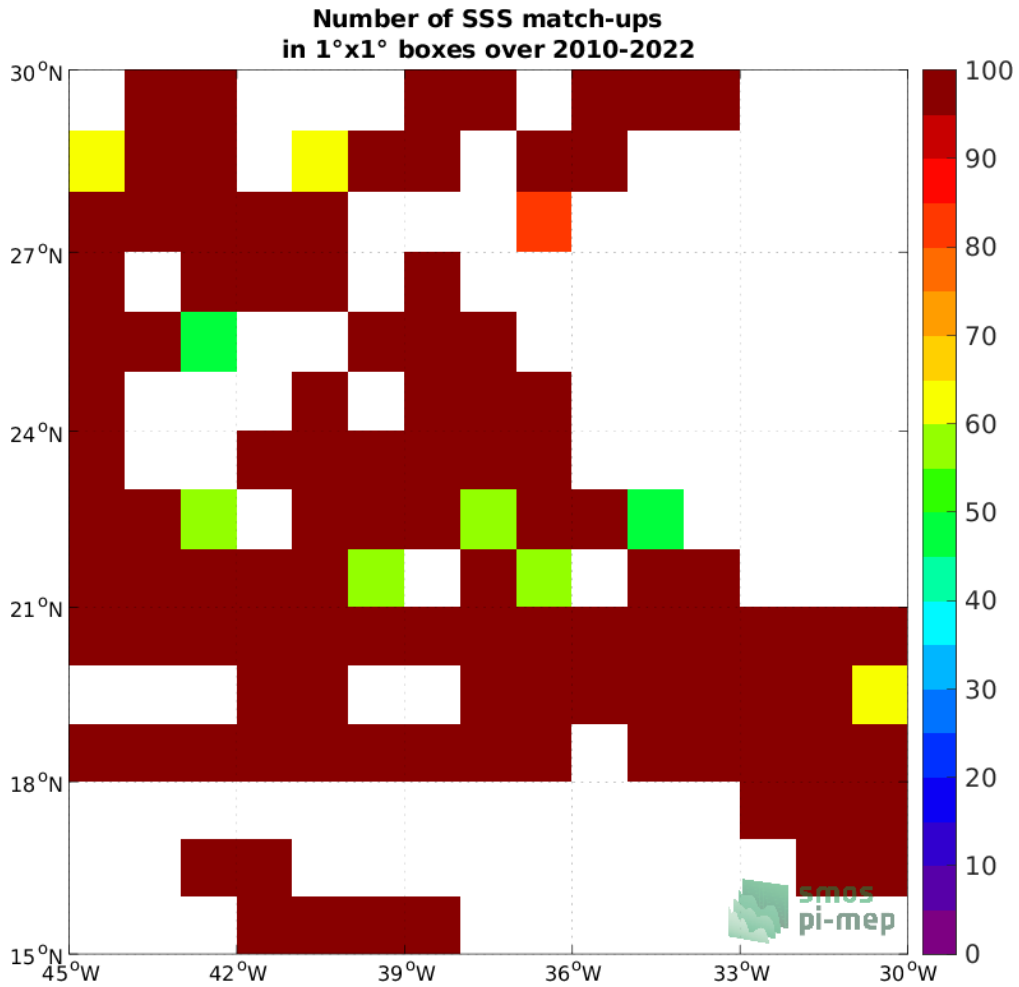
Figure 4: Number of SSS match-ups between TSG (SAMOS) SSS and the SMOS SSS L2Q v331 - With FLAG (CMEMS-CATDS-CPDC) SSS product for the SPURS 1 Pi-MEP region over 1^\circ \times 1^\circ boxes and for the full satellite product period.
