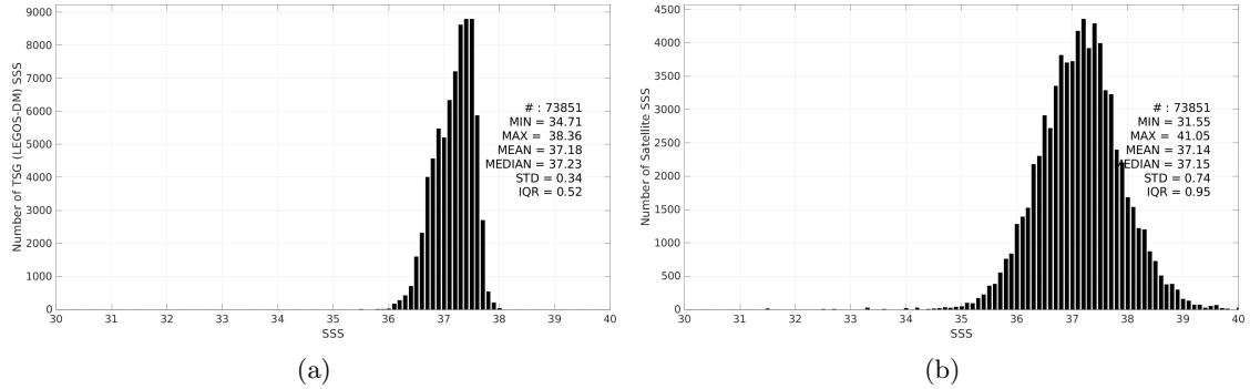
Figure 3: Histograms of SSS from TSG (LEGOS-DM) (a) and SMOS SSS L2Q v331 - With FLAG (CMEMS-CATDS-CPDC) (b) considering all match-up pairs per bins of 0.1 over the SPURS 1 Pi-MEP region and for the full satellite product period.
