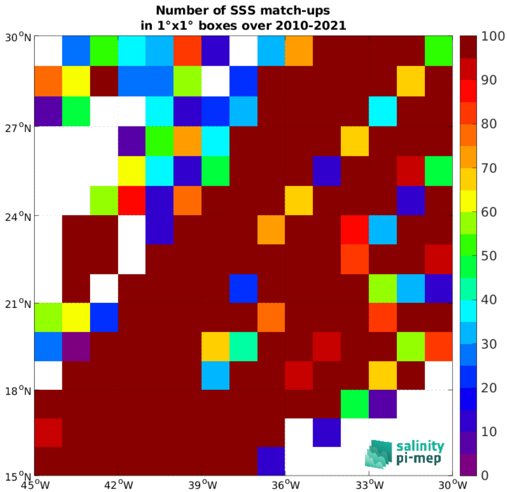
Figure 5: Number of SSS match-ups between TSG (LEGOS-DM) SSS and the SMOS SSS L2Q v331 - With FLAG (CMEMS-CATDS-CPDC) SSS product for the SPURS 1 Pi-MEP region over 1°x1° boxes and for the full satellite product period.
