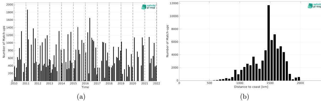
Figure 2: Number of match-ups between TSG (LEGOS-DM) and SMOS SSS L2Q v331 - With FLAG (CMEMS-CATDS-CPDC) SSS as a function of time (a) and as function of the distance to coast (b) over the SPURS 1 Pi-MEP region and for the full satellite product period.
