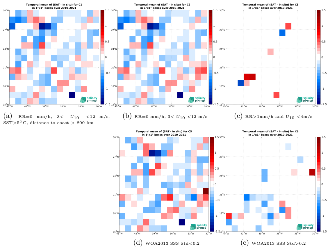
Figure 14: Temporal mean gridded over spatial boxes of size 1^\circ \times 1^\circ of \Delta SSS (SMOS SSS L2Q v331 - With FLAG (CMEMS-CATDS-CPDC) - TSG (LEGOS-DM)) for 5 different subdatasets corresponding to: RR=0 mm/h, 3 < U_{10} < 12 m/s, SST > 5^\circ\text{C} , distance to coast > 800 km (a), RR=0 mm/h, 3 < U_{10} < 12 m/s (b), RR > 1 mm/h and U_{10} < 4 m/s (c), WOA2013 SSS Std < 0.2 (d), WOA2013 SSS Std > 0.2 (e).
