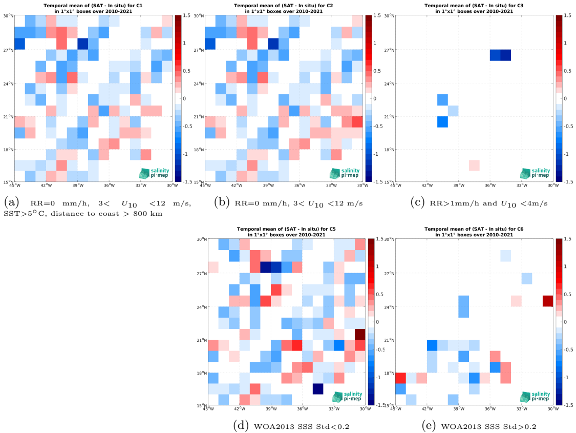
Figure 12: Temporal mean gridded over spatial boxes of size 1^{\circ}\times 1^{\circ} of \Delta\text{SSS} (SMOS SSS L2Q v331 - With FLAG (CMEMS-CATDS-CPDC) - TSG (LEGOS-DM)) for 5 different subdatasets corresponding to:RR=0 mm/h, 3 < U_{10} < 12 m/s, SST >5^{\circ}\text{C} , distance to coast > 800 km (a), RR=0 mm/h, 3 < U_{10} < 12 m/s (b), RR >1 mm/h and U_{10} < 4 m/s (c), WOA2013 SSS Std <0.2 (d), WOA2013 SSS Std >0.2 (e).
