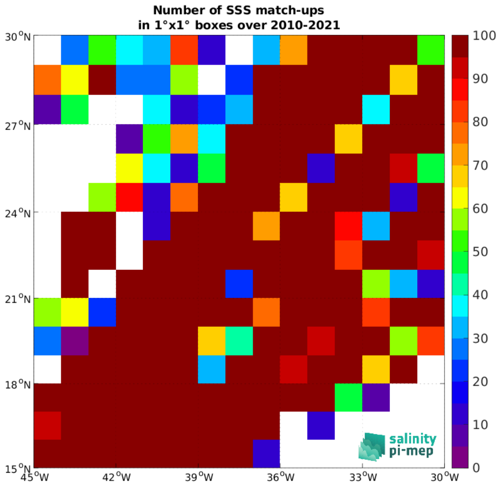
Figure 4: Number of SSS match-ups between TSG (LEGOS-DM) SSS and the SMOS SSS L2Q v331 - With FLAG (CMEMS-CATDS-CPDC) SSS product for the SPURS 1 Pi-MEP region over 1°x1° boxes and for the full satellite product period.
