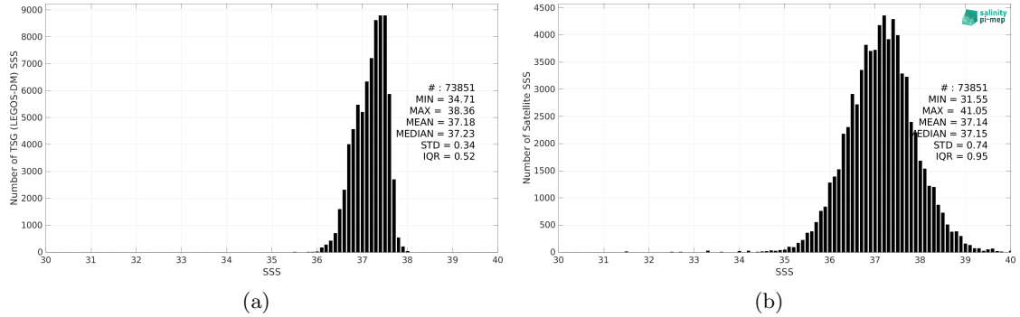
Figure 2: Histograms of SSS from TSG (LEGOS-DM) (a) and SMOS SSS L2Q v331 - With FLAG (CMEMS-CATDS-CPDC) (b) considering all match-up pairs per bins of 0.1 over the SPURS 1 Pi-MEP region and for the full satellite product period.
