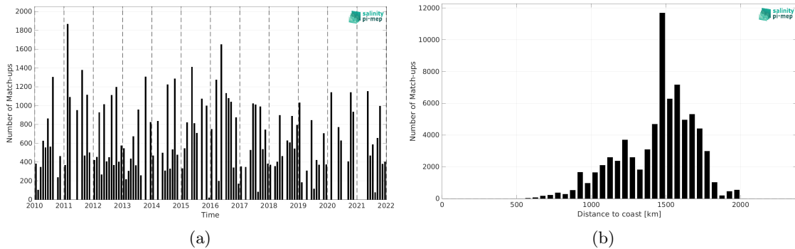
Figure 1: Number of match-ups between TSG (LEGOS-DM) and SMOS SSS L2Q v331 - With FLAG (CMEMS-CATDS-CPDC) SSS as a function of time (a) and as function of the distance to coast (b) over the SPURS 1 Pi-MEP region and for the full satellite product period.
