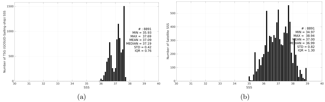
Figure 3: Histograms of SSS from TSG (GOSUD-Sailing-ship) (a) and SMOS SSS L2Q v331 - With FLAG (CMEMS-CATDS-CPDC) (b) considering all match-up pairs per bins of 0.1 over the SPURS 1 Pi-MEP region and for the full satellite product period.
