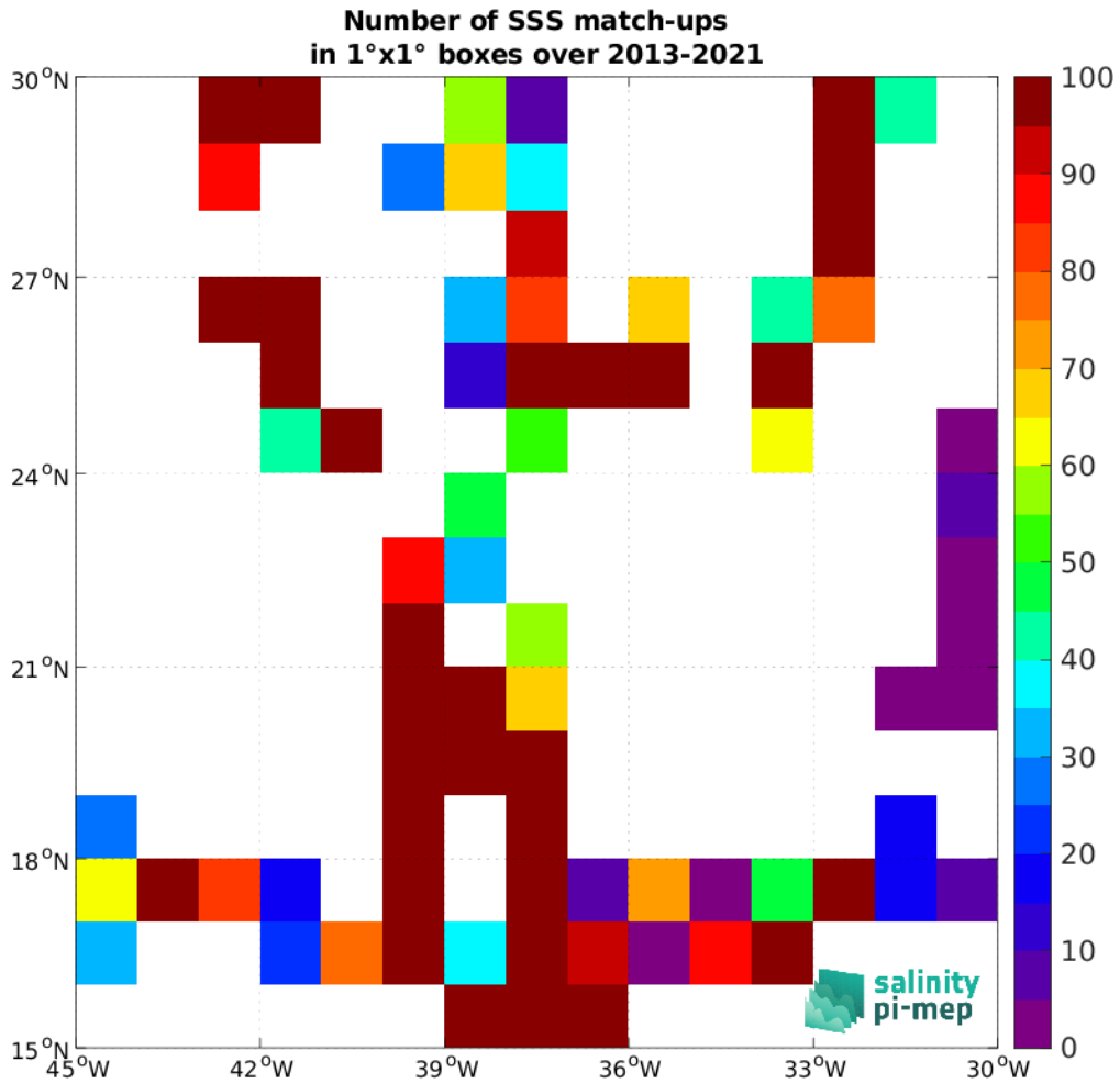
Figure 5: Number of SSS match-ups between TSG (GOSUD-Sailing-ship) SSS and the SMOS SSS L2Q v331 - With FLAG (CMEMS-CATDS-CPDC) SSS product for the SPURS 1 Pi-MEP region over 1^\circ \times 1^\circ boxes and for the full satellite product period.
