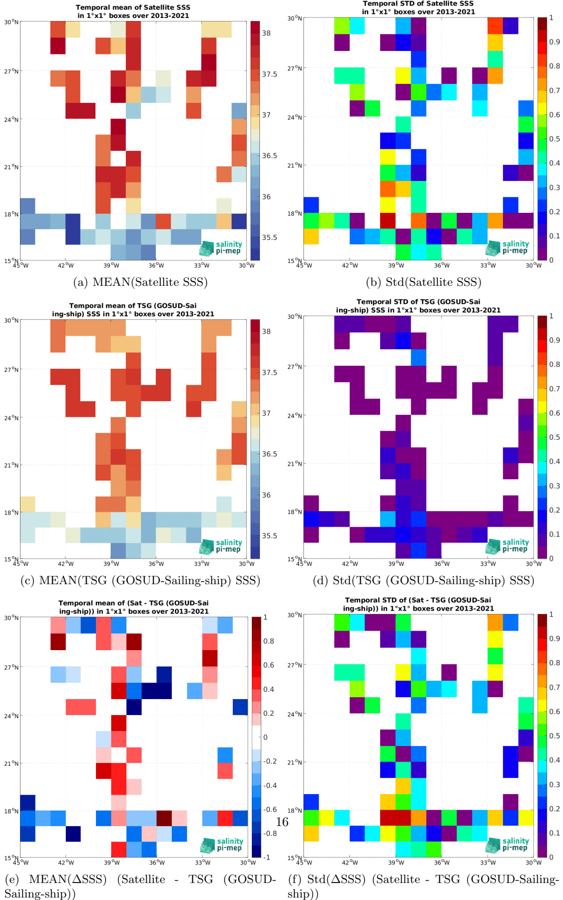
Figure 7: Temporal mean (left) and Std (right) of SSS from SMOS SSS L2Q v331 - With FLAG (CMEMS-CATDS-CPDC) (top), TSG (GOSUD-Sailing-ship) (middle), and of \Delta SSS (Satellite - TSG (GOSUD-Sailing-ship)). Only match-up pairs are used to generate these maps.
