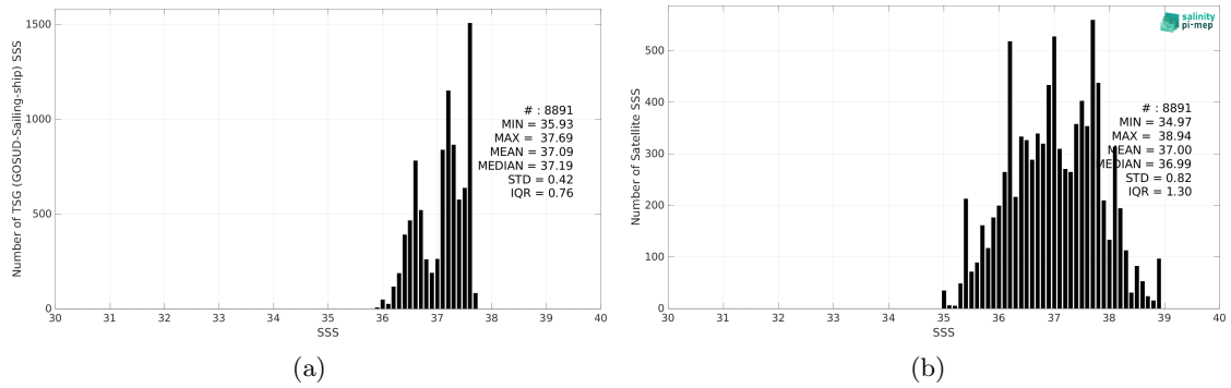
Figure 2: Histograms of SSS from TSG (GOSUD-Sailing-ship) (a) and SMOS SSS L2Q v331 - With FLAG (CMEMS-CATDS-CPDC) (b) considering all match-up pairs per bins of 0.1 over the SPURS 1 Pi-MEP region and for the full satellite product period.
