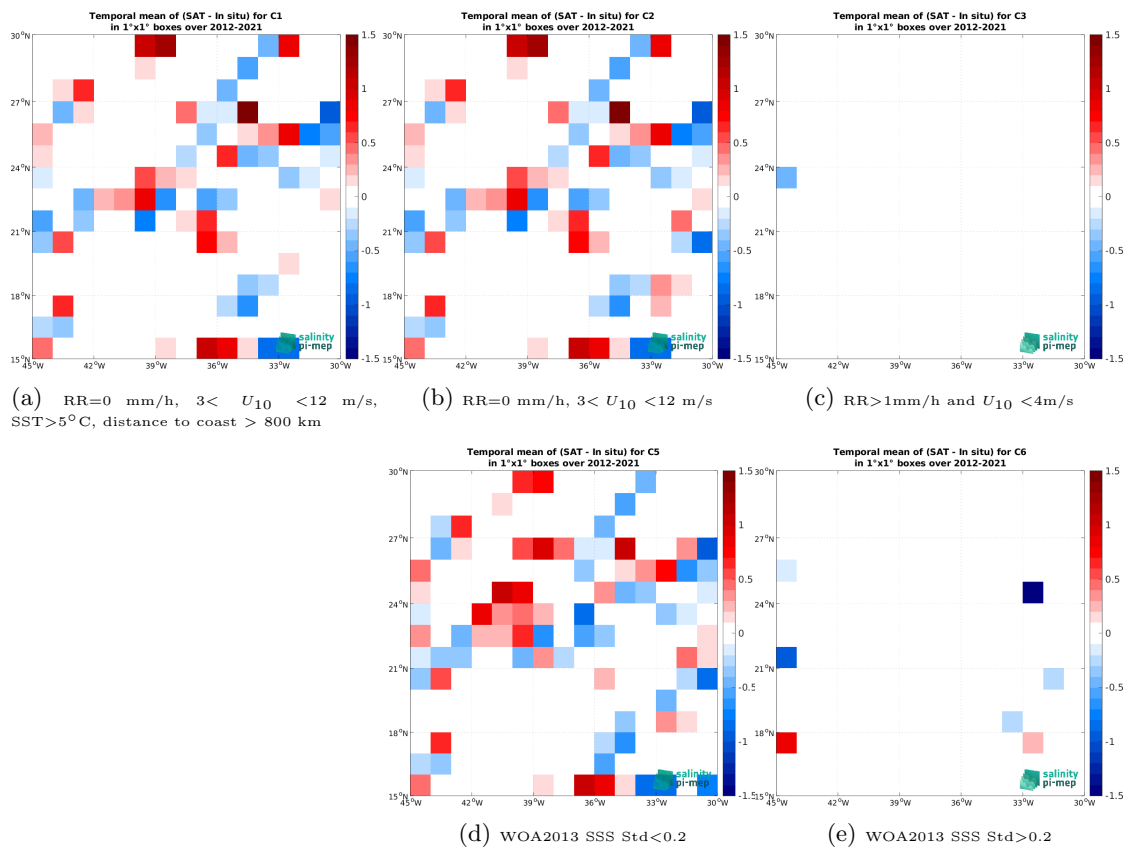
Figure 14: Temporal mean gridded over spatial boxes of size 1^\circ \times 1^\circ of \Delta SSS (SMOS SSS L2Q v331 - With FLAG (CMEMS-CATDS-CPDC) - TSG (GOSUD-Research-vessel)) for 5 different subdatasets corresponding to: RR=0 mm/h, 3 < U_{10} < 12 m/s, SST > 5^\circ C , distance to coast > 800 km (a), RR=0 mm/h, 3 < U_{10} < 12 m/s (b), RR > 1 mm/h and U_{10} < 4 m/s (c), WOA2013 SSS Std < 0.2 (d), WOA2013 SSS Std > 0.2 (e).
