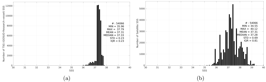
Figure 3: Histograms of SSS from TSG (GOSUD-Research-vessel) (a) and SMOS SSS L2Q v331 - With FLAG (CMEMS-CATDS-CPDC) (b) considering all match-up pairs per bins of 0.1 over the SPURS 1 Pi-MEP region and for the full satellite product period.
