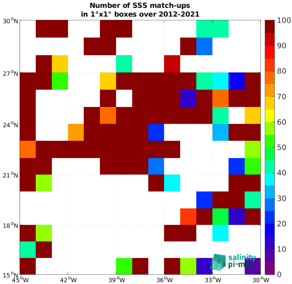
Figure 5: Number of SSS match-ups between TSG (GOSUD-Research-vessel) SSS and the SMOS SSS L2Q v331 - With FLAG (CMEMS-CATDS-CPDC) SSS product for the SPURS 1 Pi-MEP region over 1^\circ \times 1^\circ boxes and for the full satellite product period.
