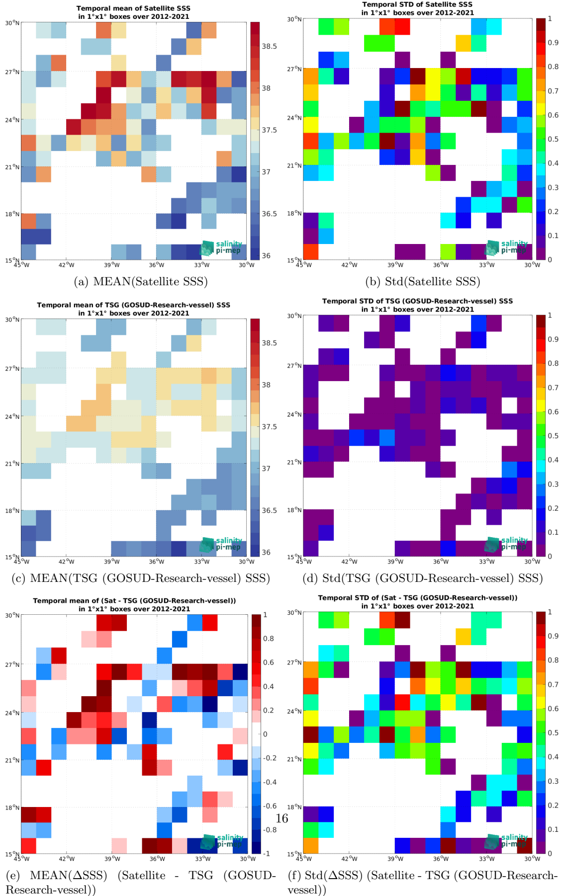
Figure 7: Temporal mean (left) and Std (right) of SSS from SMOS SSS L2Q v331 - With FLAG (CMEMS-CATDS-CPDC) (top), TSG (GOSUD-Research-vessel) (middle), and of \Delta SSS (Satellite - TSG (GOSUD-Research-vessel)). Only match-up pairs are used to generate these maps.
