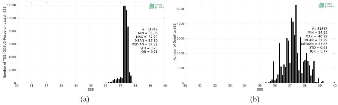
Figure 2: Histograms of SSS from TSG (GOSUD-Research-vessel) (a) and SMOS SSS L2Q v331 - With FLAG (CMEMS-CATDS-CPDC) (b) considering all match-up pairs per bins of 0.1 over the SPURS 1 Pi-MEP region and for the full satellite product period.
