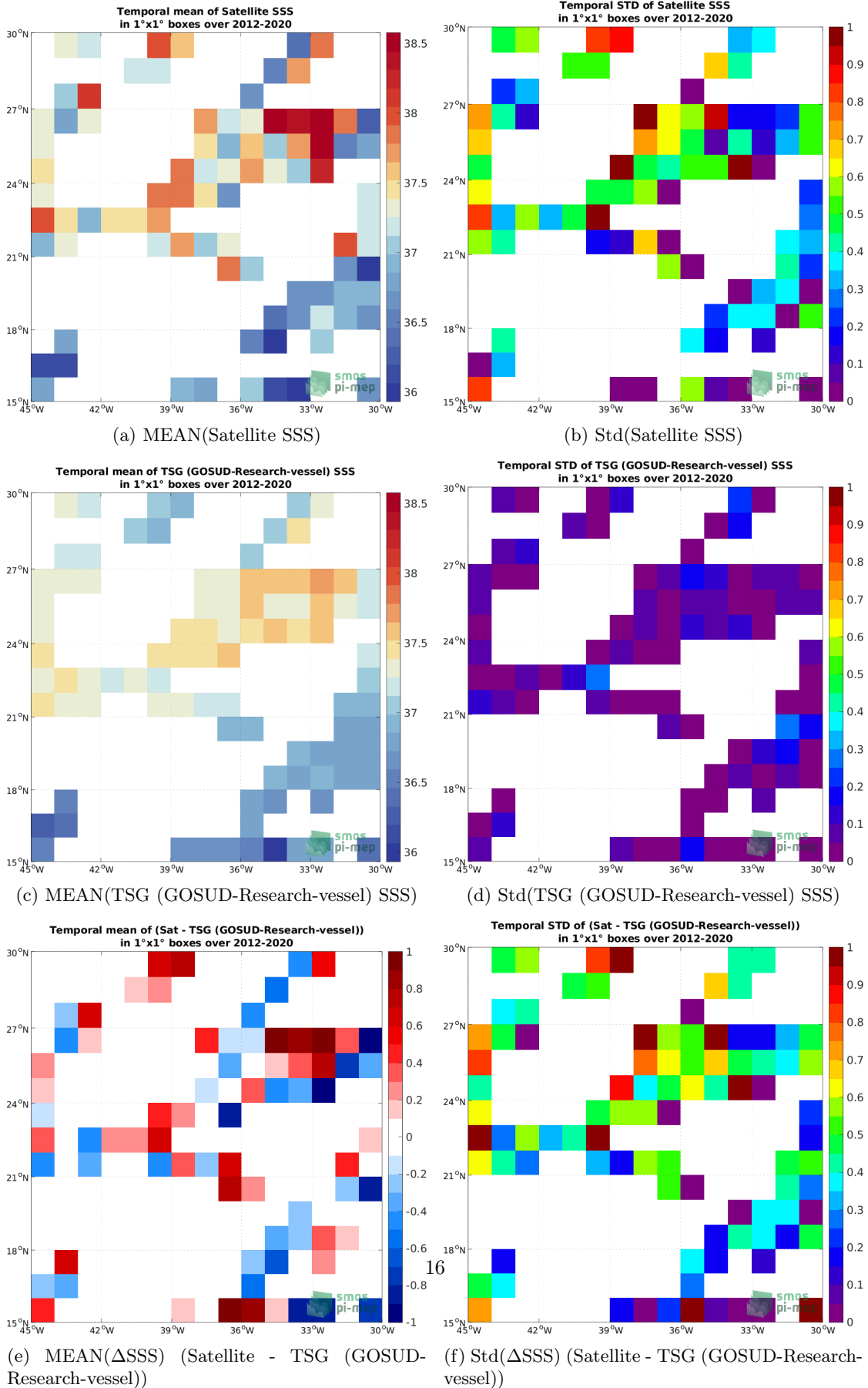
Figure 6: Temporal mean (left) and Std (right) of SSS from SMOS SSS L2Q v331 - With FLAG (CMEMS-CATDS-CPDC) (top), TSG (GOSUD-Research-vessel) (middle), and of \Delta SSS (Satellite - TSG (GOSUD-Research-vessel)). Only match-up pairs are used to generate these maps.
