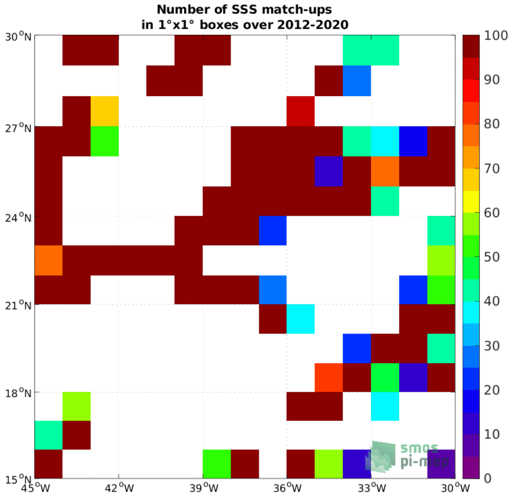
Figure 4: Number of SSS match-ups between TSG (GOSUD-Research-vessel) SSS and the SMOS SSS L2Q v331 - With FLAG (CMEMS-CATDS-CPDC) SSS product for the SPURS 1 Pi-MEP region over 1^\circ \times 1^\circ boxes and for the full satellite product period.
