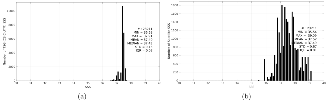
Figure 3: Histograms of SSS from TSG (CSIC-UTM) (a) and SMOS SSS L2Q v331 - With FLAG (CMEMS-CATDS-CPDC) (b) considering all match-up pairs per bins of 0.1 over the SPURS 1 Pi-MEP region and for the full satellite product period.
