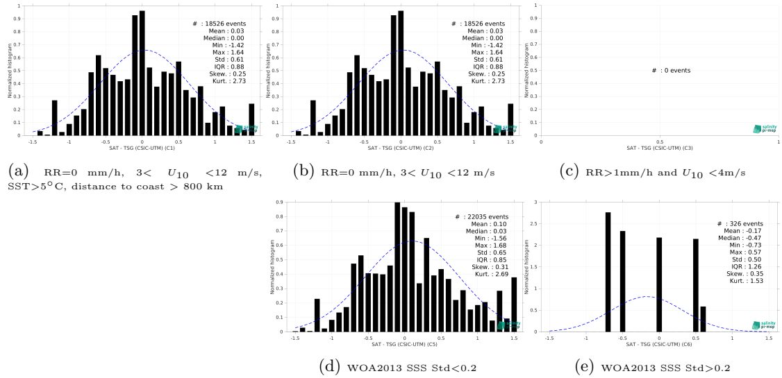
Figure 13: Normalized histogram of \Delta SSS (SMOS SSS L2Q v331 - With FLAG (CMEMS-CATDS-CPDC) - TSG (CSIC-UTM)) for 5 different subdatasets corresponding to: RR=0 mm/h, 3 < U_{10} < 12 m/s, SST > 5°C, distance to coast > 800 km (a), RR=0 mm/h, 3 < U_{10} < 12 m/s (b), RR > 1mm/h and U_{10} < 4 m/s (c), WOA2013 SSS Std < 0.2 (d), WOA2013 SSS Std > 0.2 (e).
