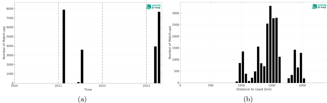
Figure 1: Number of match-ups between TSG (CSIC-UTM) and SMOS SSS L2Q v331 - With FLAG (CMEMS-CATDS-CPDC) SSS as a function of time (a) and as function of the distance to coast (b) over the SPURS 1 Pi-MEP region and for the full satellite product period.
