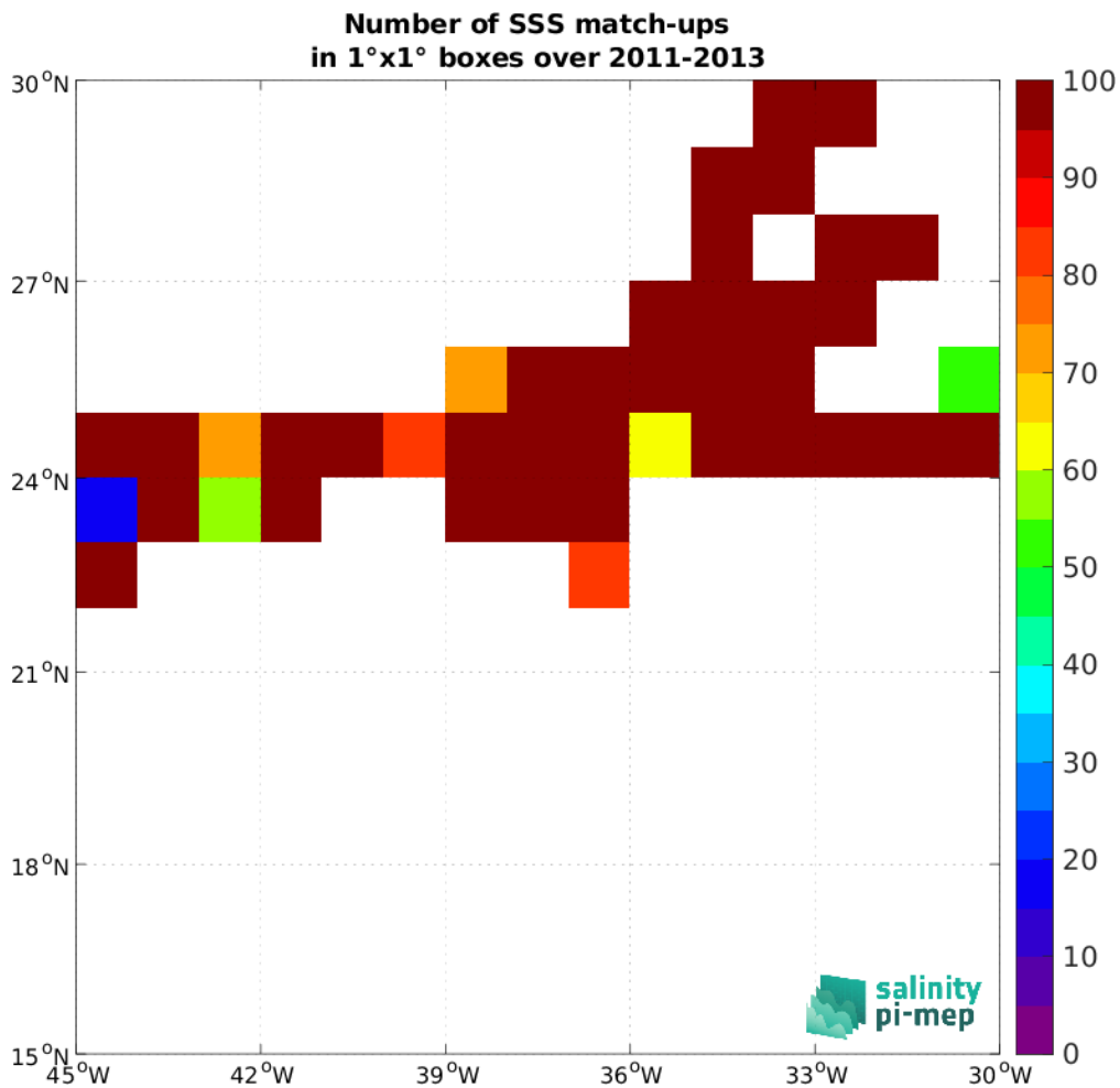
Figure 4: Number of SSS match-ups between TSG (CSIC-UTM) SSS and the SMOS SSS L2Q v331 - With FLAG (CMEMS-CATDS-CPDC) SSS product for the SPURS 1 Pi-MEP region over 1^\circ \times 1^\circ boxes and for the full satellite product period.
