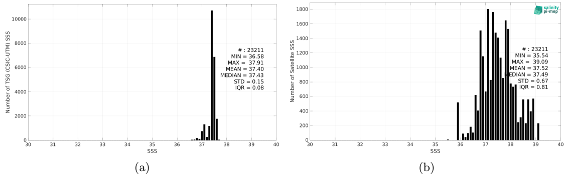
Figure 2: Histograms of SSS from TSG (CSIC-UTM) (a) and SMOS SSS L2Q v331 - With FLAG (CMEMS-CATDS-CPDC) (b) considering all match-up pairs per bins of 0.1 over the SPURS 1 Pi-MEP region and for the full satellite product period.
