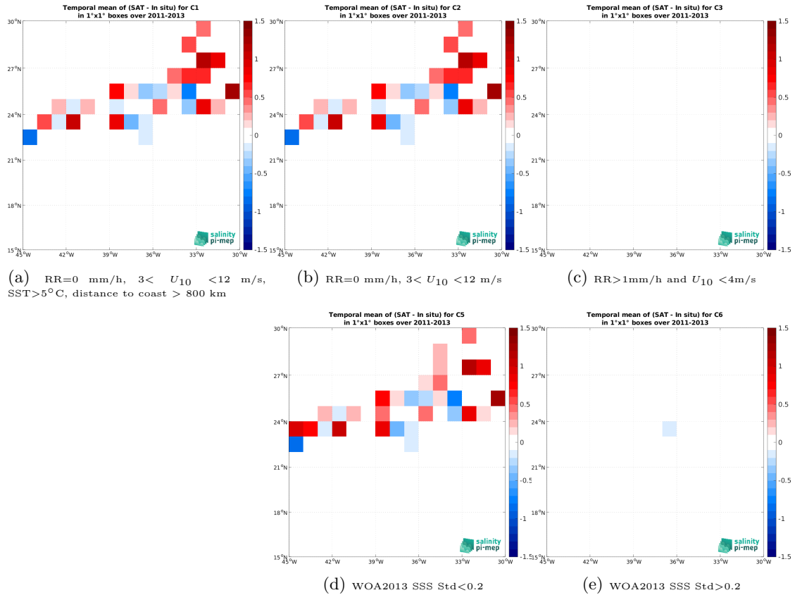
Figure 12: Temporal mean gridded over spatial boxes of size 1^{\circ}\times 1^{\circ} of \Delta\text{SSS} (SMOS SSS L2Q v331 - With FLAG (CMEMS-CATDS-CPDC) - TSG (CSIC-UTM)) for 5 different subdatasets corresponding to:RR=0 mm/h, 3 < U_{10} < 12 m/s, SST >5^{\circ}\text{C} , distance to coast > 800 km (a), RR=0 mm/h, 3 < U_{10} < 12 m/s (b), RR >1 mm/h and U_{10} < 4 m/s (c), WOA2013 SSS Std <0.2 (d), WOA2013 SSS Std >0.2 (e).
