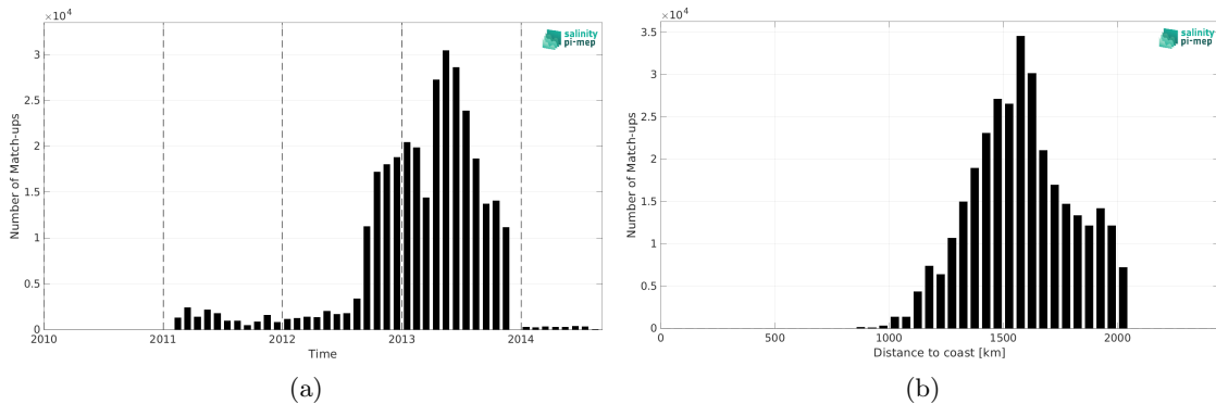
Figure 2: Number of match-ups between Surface drifters and SMOS SSS L2Q v331 - With FLAG (CMEMS-CATDS-CPDC) SSS as a function of time (a) and as function of the distance to coast (b) over the SPURS 1 Pi-MEP region and for the full satellite product period.
