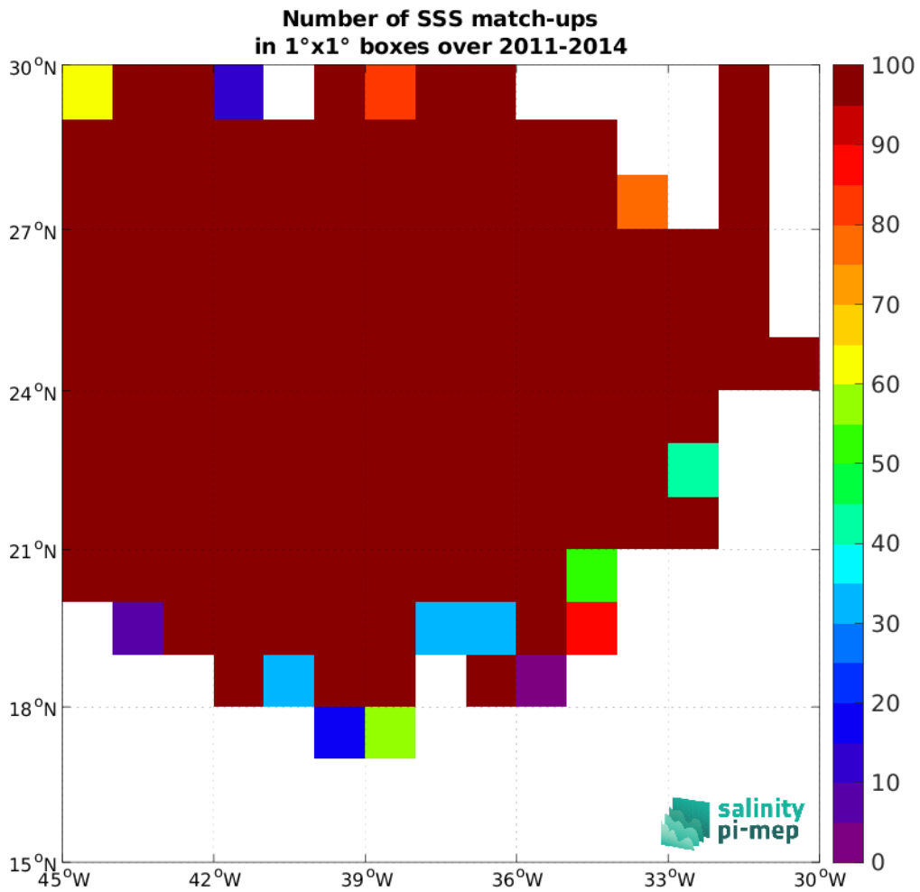
Figure 4: Number of SSS match-ups between Surface drifters SSS and the SMOS SSS L2Q v331 - With FLAG (CMEMS-CATDS-CPDC) SSS product for the SPURS 1 Pi-MEP region over 1°×1° boxes and for the full satellite product period.
