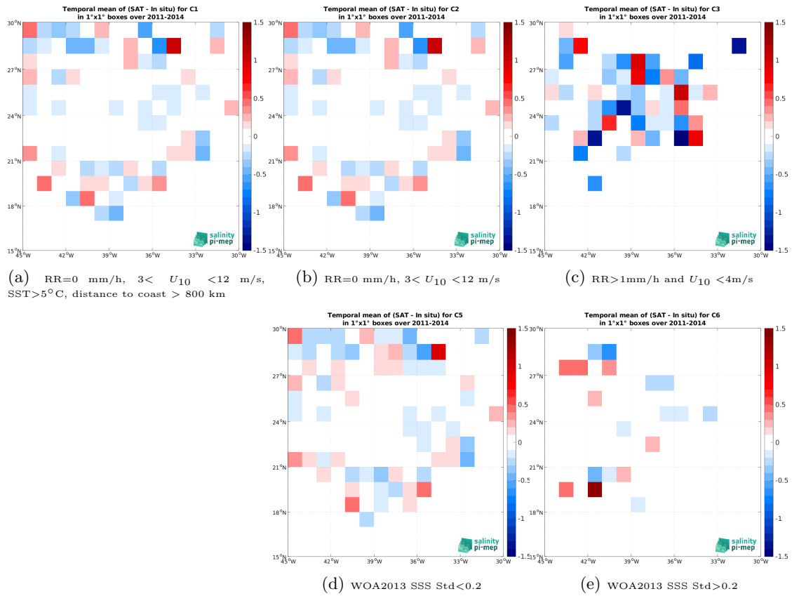
Figure 13: Temporal mean gridded over spatial boxes of size 1^\circ \times 1^\circ of \Delta SSS (SMOS SSS L2Q v331 - With FLAG (CMEMS-CATDS-CPDC) - Surface drifters) for 5 different subdatasets corresponding to:RR=0 mm/h, 3 < U_{10} < 12 m/s, SST >5^\circ C, distance to coast > 800 km (a), RR=0 mm/h, 3 < U_{10} < 12 m/s (b), RR >1 mm/h and U_{10} < 4 m/s (c), WOA2013 SSS Std <0.2 (d), WOA2013 SSS Std >0.2 (e).
