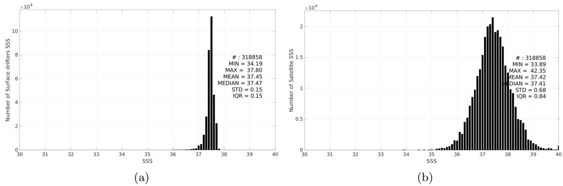
Figure 3: Histograms of SSS from Surface drifters (a) and SMOS SSS L2Q v331 - With FLAG (CMEMS-CATDS-CPDC) (b) considering all match-up pairs per bins of 0.1 over the SPURS 1 Pi-MEP region and for the full satellite product period.
