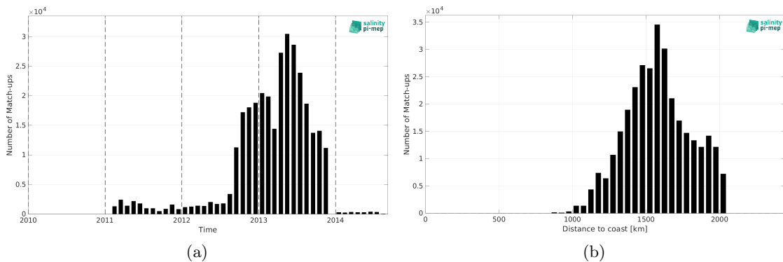
Figure 1: Number of match-ups between Surface drifters and SMOS SSS L2Q v331 - With FLAG (CMEMS-CATDS-CPDC) SSS as a function of time (a) and as function of the distance to coast (b) over the SPURS 1 Pi-MEP region and for the full satellite product period.
