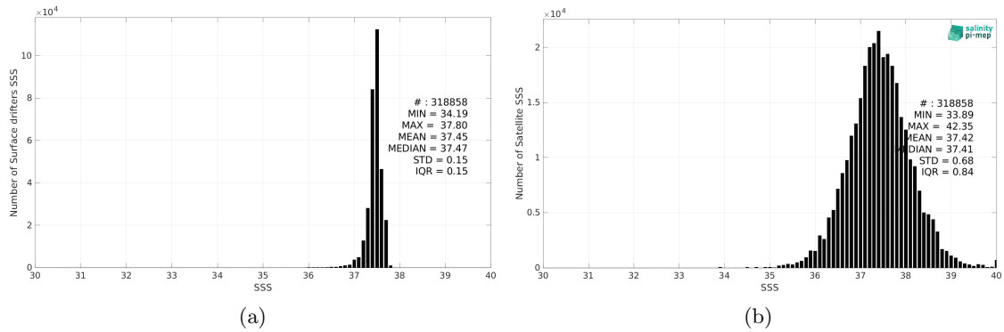
Figure 2: Histograms of SSS from Surface drifters (a) and SMOS SSS L2Q v331 - With FLAG (CMEMS-CATDS-CPDC) (b) considering all match-up pairs per bins of 0.1 over the SPURS 1 Pi-MEP region and for the full satellite product period.
