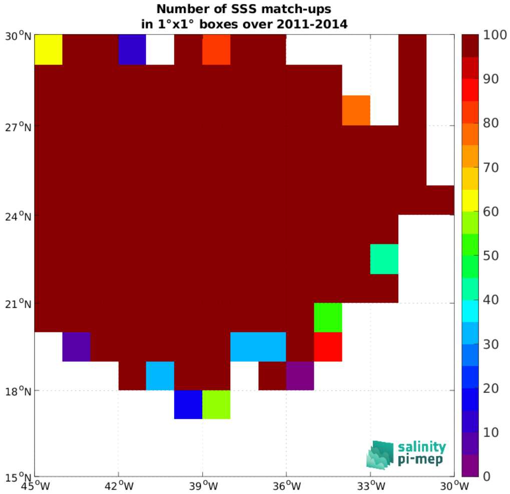
Figure 3: Number of SSS match-ups between Surface drifters SSS and the SMOS SSS L2Q v331 - With FLAG (CMEMS-CATDS-CPDC) SSS product for the SPURS 1 Pi-MEP region over 1^\circ \times 1^\circ boxes and for the full satellite product period.
