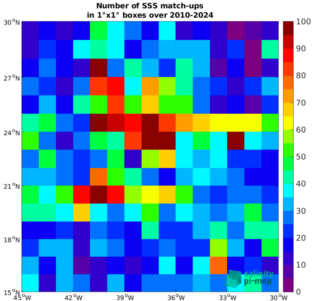
Figure 5: Number of SSS match-ups between Argo SSS and the SMOS SSS L2Q v331 - With FLAG (CMEMS-CATDS-CPDC) SSS product for the SPURS 1 Pi-MEP region over 1^\circ \times 1^\circ boxes and for the full satellite product period.
