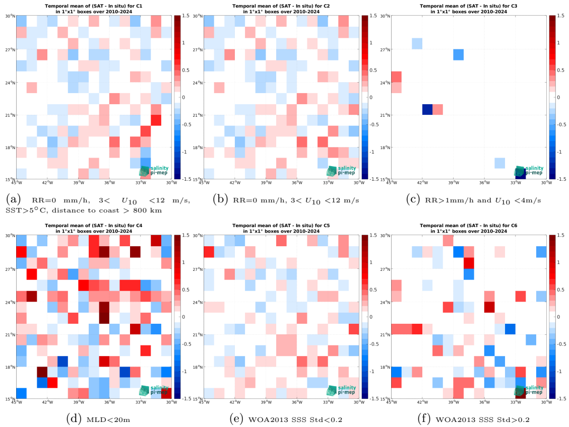
Figure 14: Temporal mean gridded over spatial boxes of size 1^\circ \times 1^\circ of \Delta SSS (SMOS SSS L2Q v331 - With FLAG (CMEMS-CATDS-CPDC) - Argo) for 6 different subdatasets corresponding to:RR=0 mm/h, 3 < U_{10} < 12 m/s, SST >5^\circ C, distance to coast > 800 km (a), RR=0 mm/h, 3 < U_{10} < 12 m/s (b), RR >1 mm/h and U_{10} < 4 m/s (c),MLD <20 m (d),WOA2013 SSS Std <0.2 (e),WOA2013 SSS Std >0.2 (f).
