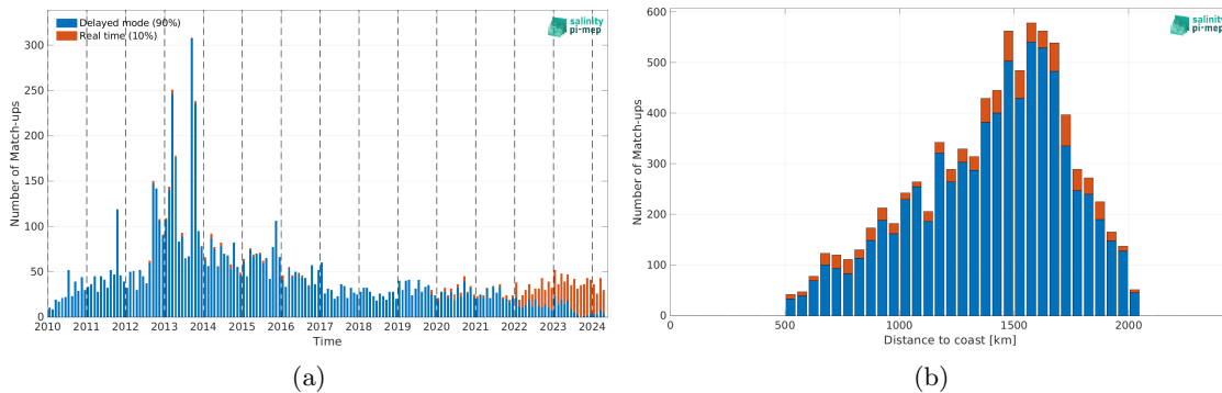
Figure 2: Number of match-ups between Argo and SMOS SSS L2Q v331 - With FLAG (CMEMS-CATDS-CPDC) SSS as a function of time (a) and as function of the distance to coast (b) over the SPURS 1 Pi-MEP region and for the full satellite product period.
