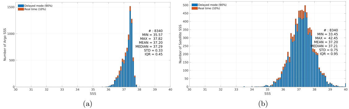
Figure 3: Histograms of SSS from Argo (a) and SMOS SSS L2Q v331 - With FLAG (CMEMS-CATDS-CPDC) (b) considering all match-up pairs per bins of 0.1 over the SPURS 1 Pi-MEP region and for the full satellite product period.
