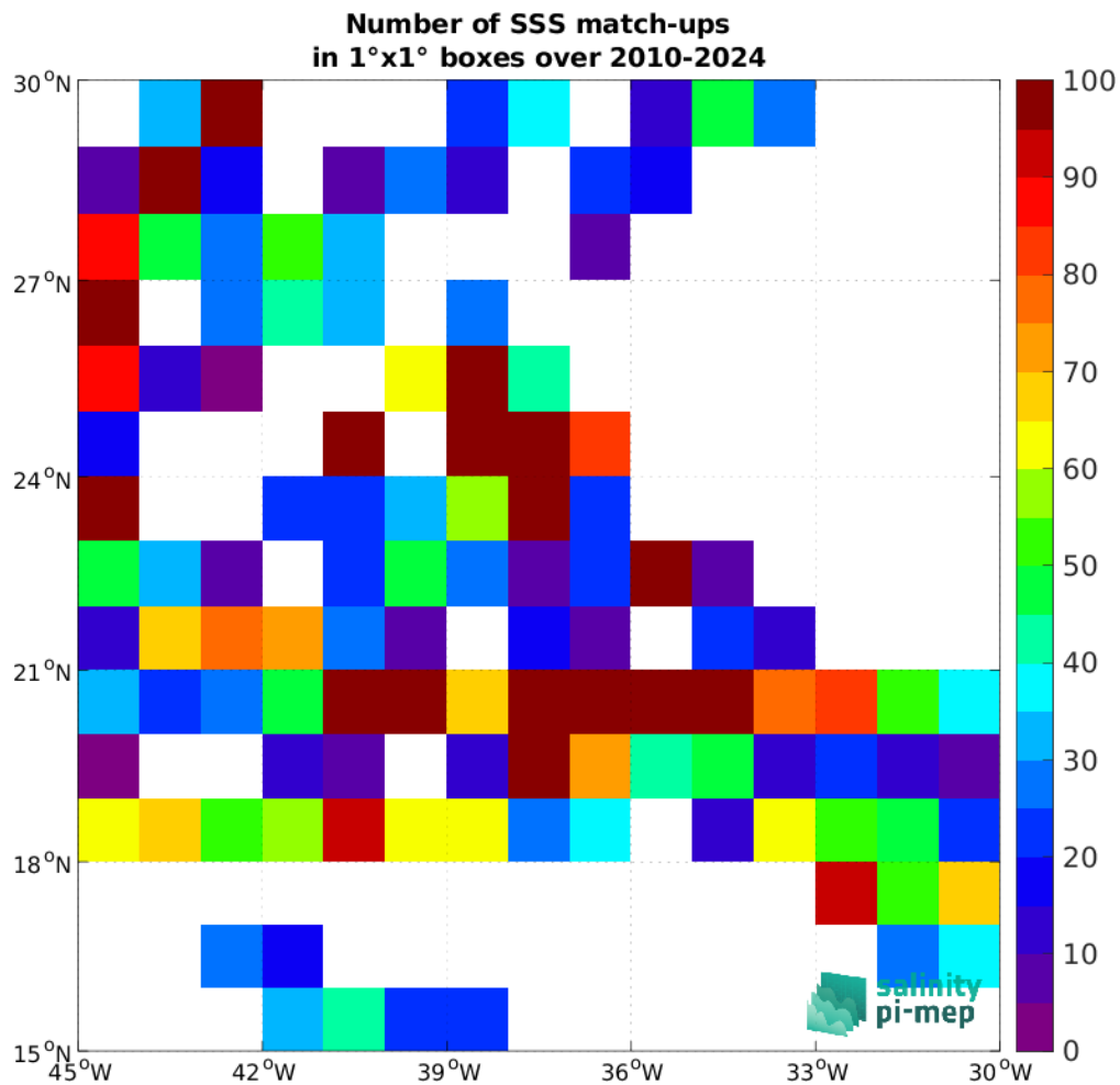
Figure 5: Number of SSS match-ups between TSG (SAMOS) SSS and the SMOS SSS L2Q v331 - No FLAG (CMEMS-CATDS-CPDC) SSS product for the SPURS 1 Pi-MEP region over 1°x1° boxes and for the full satellite product period.
