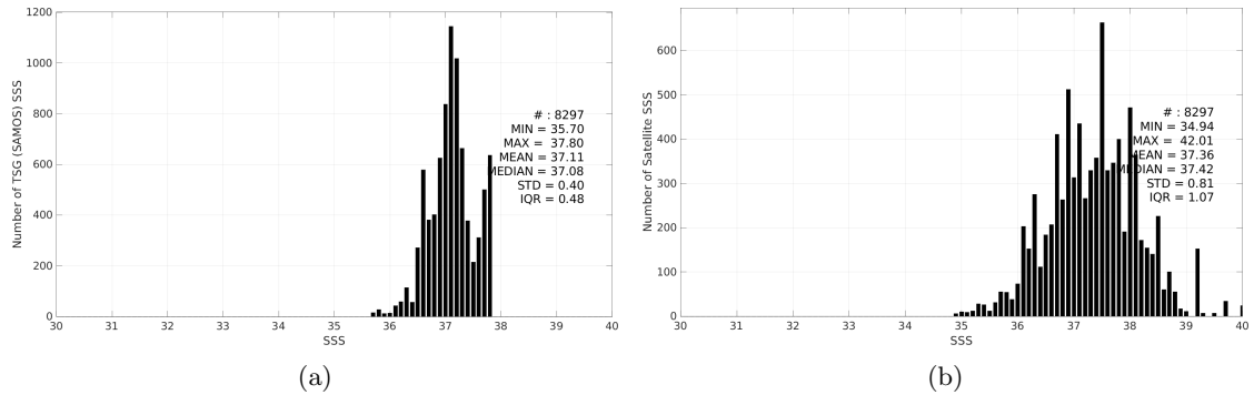
Figure 3: Histograms of SSS from TSG (SAMOS) (a) and SMOS SSS L2Q v331 - No FLAG (CMEMS-CATDS-CPDC) (b) considering all match-up pairs per bins of 0.1 over the SPURS 1 Pi-MEP region and for the full satellite product period.
