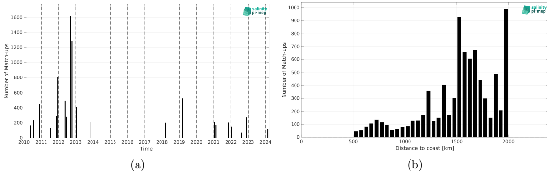
Figure 2: Number of match-ups between TSG (SAMOS) and SMOS SSS L2Q v331 - No FLAG (CMEMS-CATDS-CPDC) SSS as a function of time (a) and as function of the distance to coast (b) over the SPURS 1 Pi-MEP region and for the full satellite product period.
