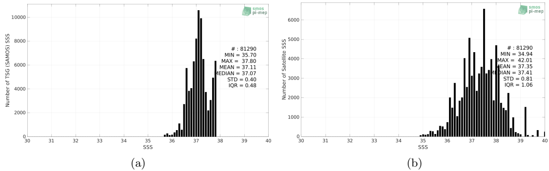
Figure 2: Histograms of SSS from TSG (SAMOS) (a) and SMOS SSS L2Q v331 - No FLAG (CMEMS-CATDS-CPDC) (b) considering all match-up pairs per bins of 0.1 over the SPURS 1 Pi-MEP region and for the full satellite product period.
