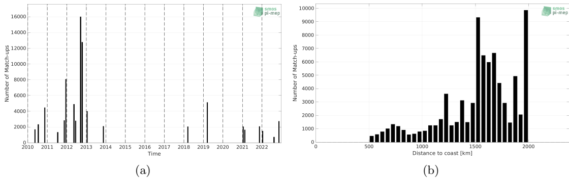
Figure 1: Number of match-ups between TSG (SAMOS) and SMOS SSS L2Q v331 - No FLAG (CMEMS-CATDS-CPDC) SSS as a function of time (a) and as function of the distance to coast (b) over the SPURS 1 Pi-MEP region and for the full satellite product period.
