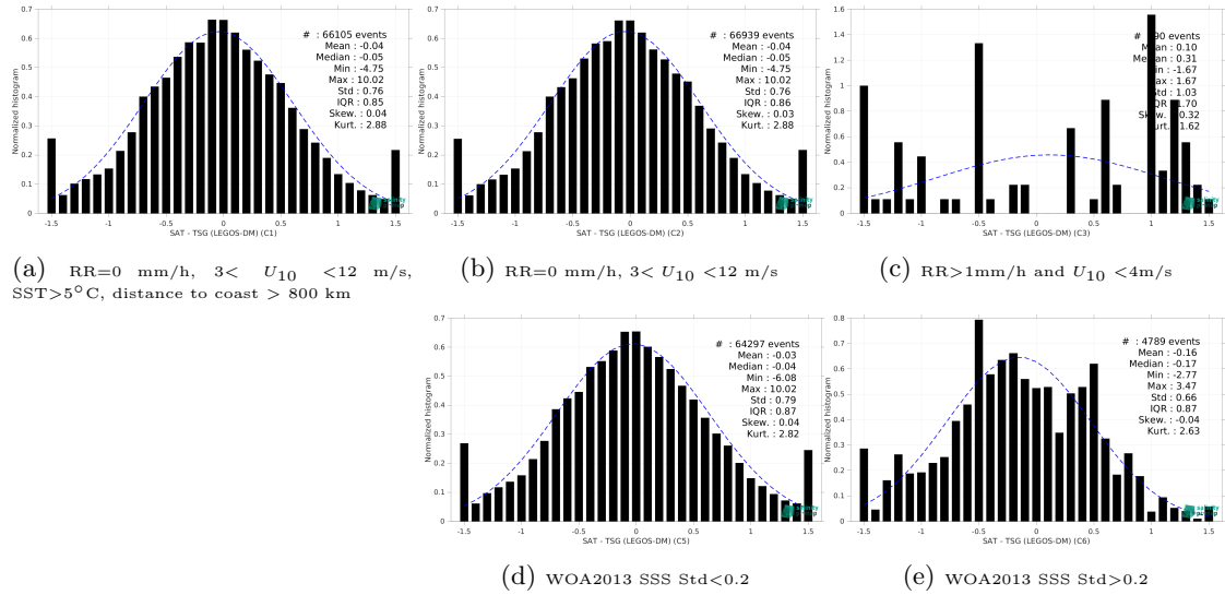
Figure 15: Normalized histogram of \Delta\text{SSS} (SMOS SSS L2Q v331 - No FLAG (CMEMS-CATDS-CPDC) - TSG (LEGOS-DM)) for 5 different subdatasets corresponding to: RR=0 mm/h, 3 < U_{10} < 12 m/s, SST>5°C, distance to coast > 800 km (a), RR=0 mm/h, 3 < U_{10} < 12 m/s (b), RR>1mm/h and U_{10} < 4 m/s (c), WOA2013 SSS Std<0.2 (d), WOA2013 SSS Std>0.2 (e).
