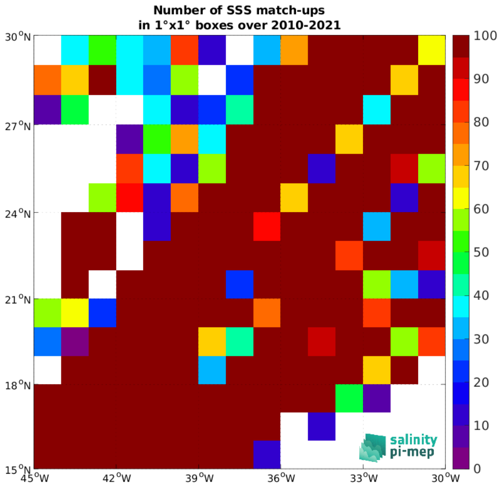
Figure 5: Number of SSS match-ups between TSG (LEGOS-DM) SSS and the SMOS SSS L2Q v331 - No FLAG (CMEMS-CATDS-CPDC) SSS product for the SPURS 1 Pi-MEP region over 1^\circ \times 1^\circ boxes and for the full satellite product period.
