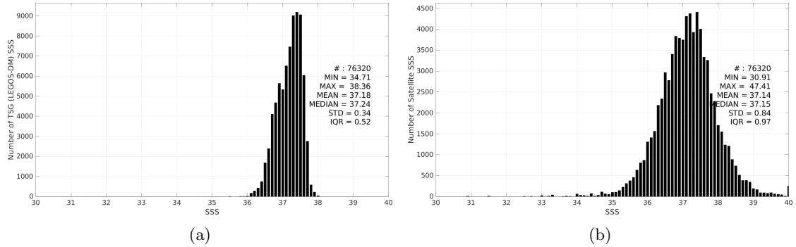
Figure 3: Histograms of SSS from TSG (LEGOS-DM) (a) and SMOS SSS L2Q v331 - No FLAG (CMEMS-CATDS-CPDC) (b) considering all match-up pairs per bins of 0.1 over the SPURS 1 Pi-MEP region and for the full satellite product period.
