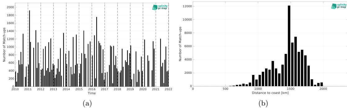
Figure 2: Number of match-ups between TSG (LEGOS-DM) and SMOS SSS L2Q v331 - No FLAG (CMEMS-CATDS-CPDC) SSS as a function of time (a) and as function of the distance to coast (b) over the SPURS 1 Pi-MEP region and for the full satellite product period.
