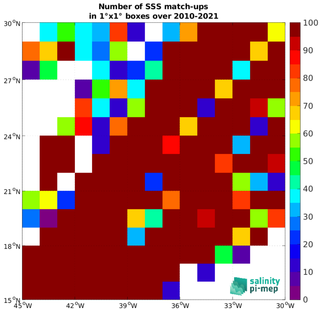
Figure 4: Number of SSS match-ups between TSG (LEGOS-DM) SSS and the SMOS SSS L2Q v331 - No FLAG (CMEMS-CATDS-CPDC) SSS product for the SPURS 1 Pi-MEP region over 1^\circ \times 1^\circ boxes and for the full satellite product period.
