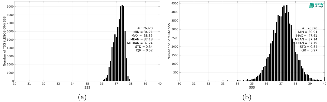
Figure 2: Histograms of SSS from TSG (LEGOS-DM) (a) and SMOS SSS L2Q v331 - No FLAG (CMEMS-CATDS-CPDC) (b) considering all match-up pairs per bins of 0.1 over the SPURS 1 Pi-MEP region and for the full satellite product period.
