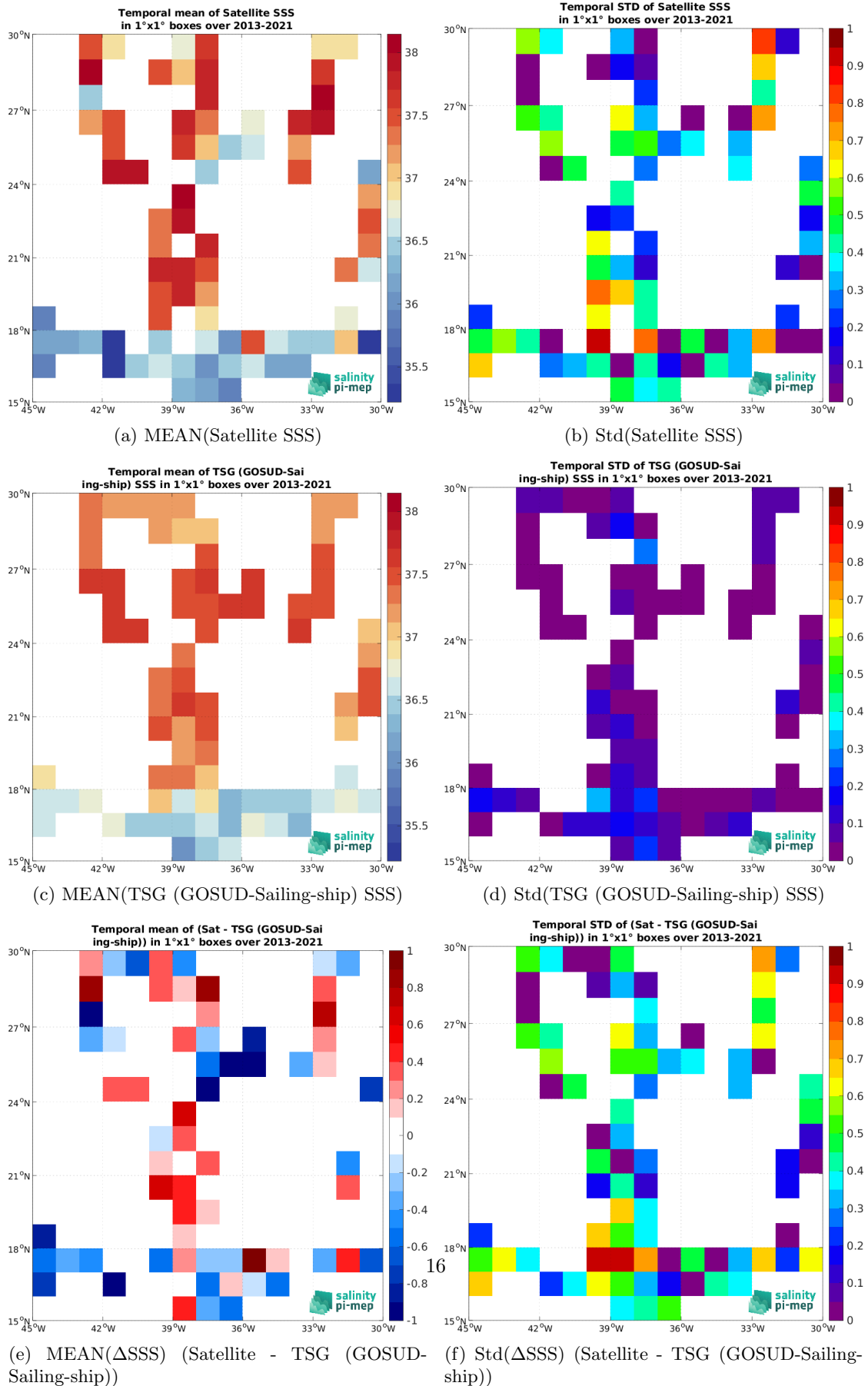
Figure 7: Temporal mean (left) and Std (right) of SSS from SMOS SSS L2Q v331 - No FLAG (CMEMS-CATDS-CPDC) (top), TSG (GOSUD-Sailing-ship) (middle), and of \Delta SSS (Satellite - TSG (GOSUD-Sailing-ship)). Only match-up pairs are used to generate these maps.
