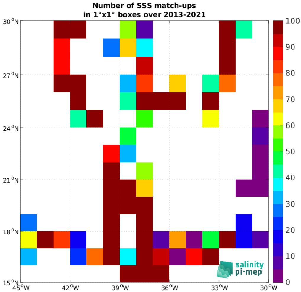
Figure 5: Number of SSS match-ups between TSG (GOSUD-Sailing-ship) SSS and the SMOS SSS L2Q v331 - No FLAG (CMEMS-CATDS-CPDC) SSS product for the SPURS 1 Pi-MEP region over 1^\circ \times 1^\circ boxes and for the full satellite product period.
