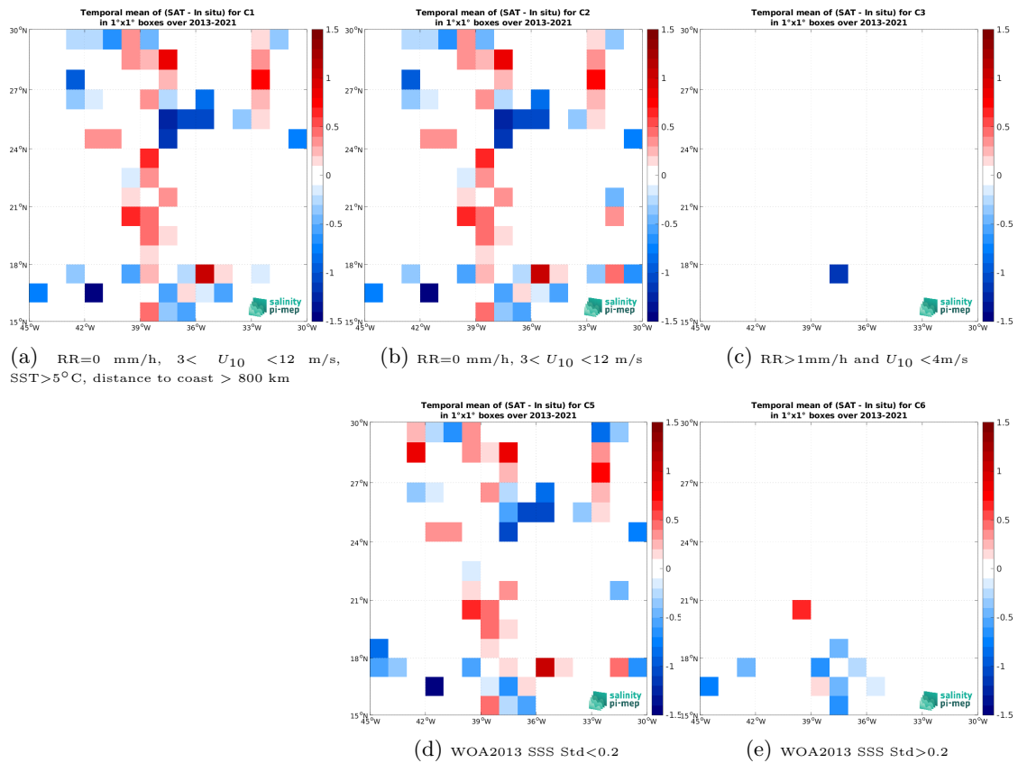
Figure 14: Temporal mean gridded over spatial boxes of size 1^\circ \times 1^\circ of \Delta\text{SSS} (SMOS SSS L2Q v331 - No FLAG (CMEMS-CATDS-CPDC) - TSG (GOSUD-Sailing-ship)) for 5 different sub-datasets corresponding to:RR=0 mm/h, 3 < U_{10} < 12 m/s, SST>5°C, distance to coast > 800 km (a), RR=0 mm/h, 3 < U_{10} < 12 m/s (b), RR>1mm/h and U_{10} < 4 m/s (c), WOA2013 SSS Std<0.2 (d), WOA2013 SSS Std>0.2 (e).
