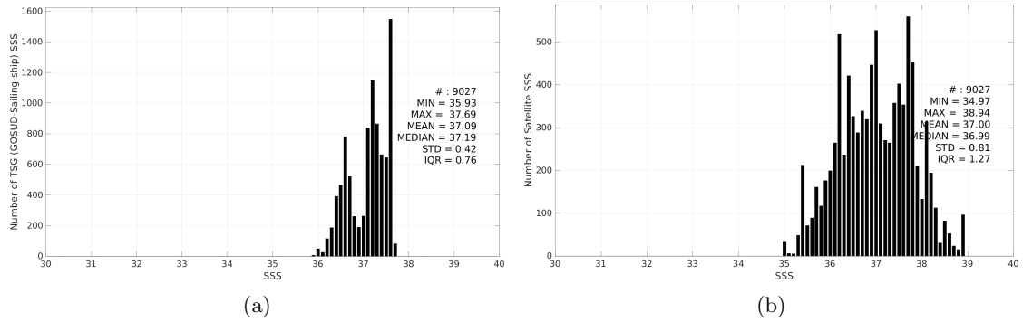
Figure 3: Histograms of SSS from TSG (GOSUD-Sailing-ship) (a) and SMOS SSS L2Q v331 - No FLAG (CMEMS-CATDS-CPDC) (b) considering all match-up pairs per bins of 0.1 over the SPURS 1 Pi-MEP region and for the full satellite product period.
